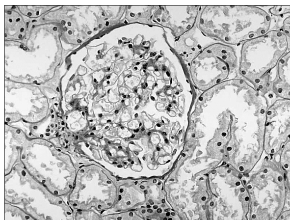
Figure 3. Overall architecture of the glomeruli was well preserved and capillary loops were intact and patent (H&E stain, ×400).
