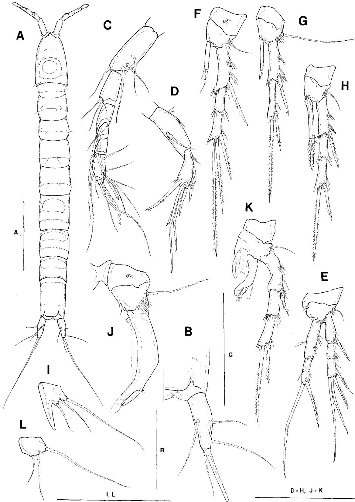
Fig. 6. Parastenocaris brevipes . A-I, female: A, habitus, dorsal; B, anal somite and caudal rami, dorsal; C, antennule; D, antenna; E-I, legs 1-5. J-L, male legs 3-5. Scale bars: A=100 μm, B-L=50 μm.
