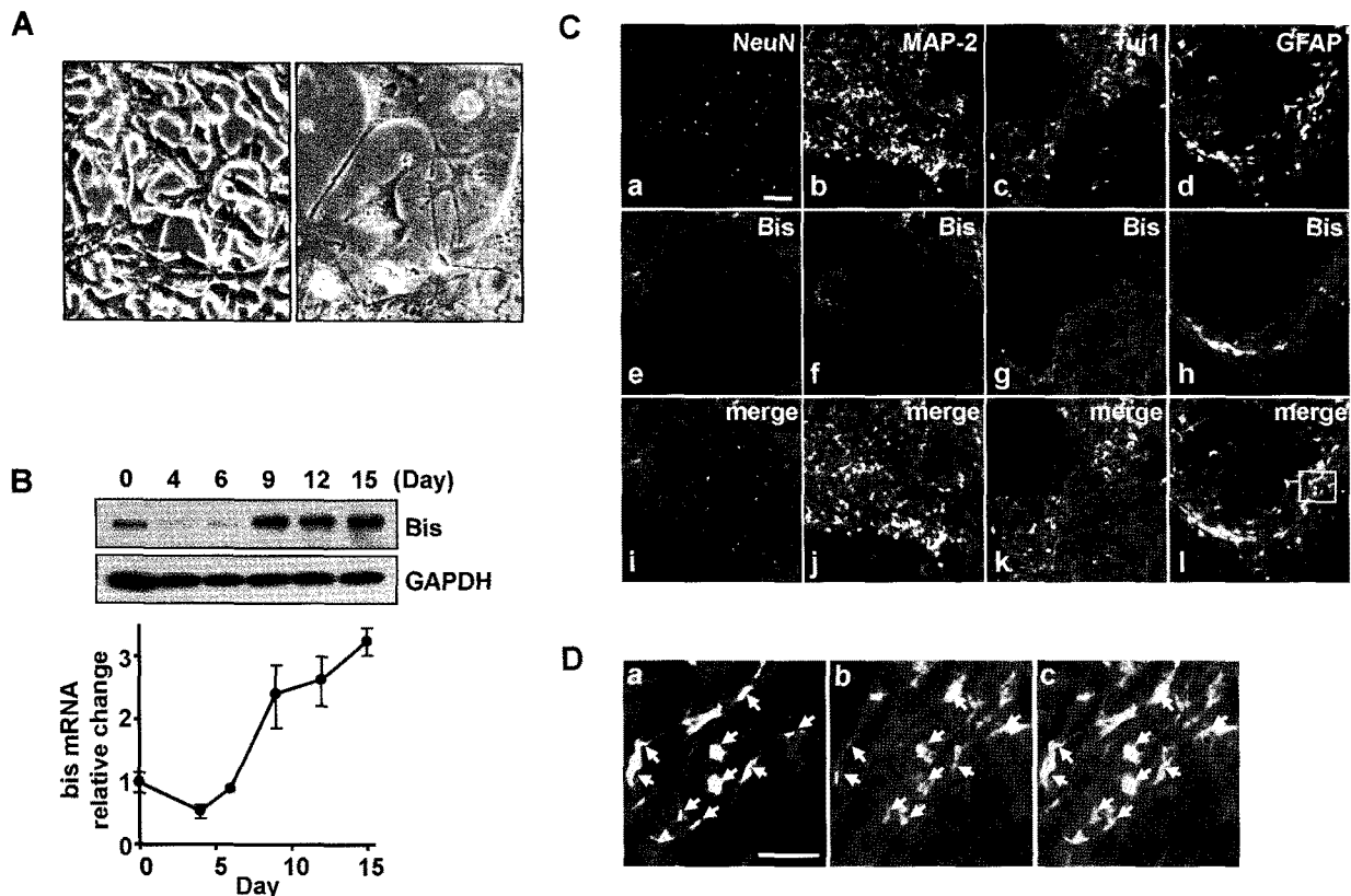
Fig. 1. Expression of Bis in GFAP-positive glia cells during RA-induced differentiation in P19 cells. (A) Light microscopic images of P19 cells before (left) and after (right) the induction of neuronal differentiation (day 12). (B) Change in Bis protein levels during the RA-induced differentiation of P19 cells was examined by immunoblotting (upper panel). The expression of GAPDH is shown as a loading control. The relative expression of bis mRNA levels was determined by real-time RT-PCR after normalizing to endogenous GAPDH control (lower graph). The value at day 0 was arbitrarily designated as 1.0. (C) Confocal laser microscopic imaging of immunofluorescence for Bis (e–h) and one of the marker antibodies for NeuN (a), MAP-2 (b), Tuj-1 (c) and GFAP (d) at day 12 after the induction of neuronal differentiation. (i–l) Superimposed images of FITC (a–d) and Cy3 (e–h). Scale bar, 50 \mu m. (D) Higher magnification of the boxed area in (C). Most GFAP labeled cells were immunoreactive for Bis (arrows in panel a–c). Scale bar, 20 \mu m.
