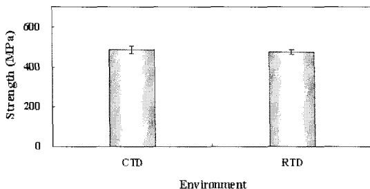
Fig. 5 Open hole tensile strengths of pattern_2 specimens for W/D=6.
