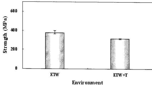
Fig. 13 Filled hole compressive strengths of pattern_2 specimens for W/D=6.
