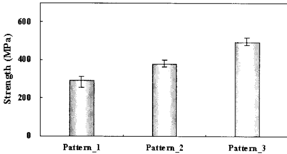
Fig. 16 Filled hole compressive strengths of specimens for ETW and W/D=6 as a function of pattern.
