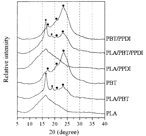
Fig. 7 WAXD curves of PLA/PBT/PPDI samples annealed at 75°C for 30 min.
