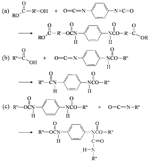
Fig. 4 Anticipated reactions of chain extension among PLA, PBT, and PPDI with the formation of (a) urethane bonds, (b) amide bonds, and (c) allophanate bonds. R is H or CH 3 , R' is the repeating unit of PLA or PBT, and R'' represents the bonds reacted among PLA, PBT, and PPDI.
