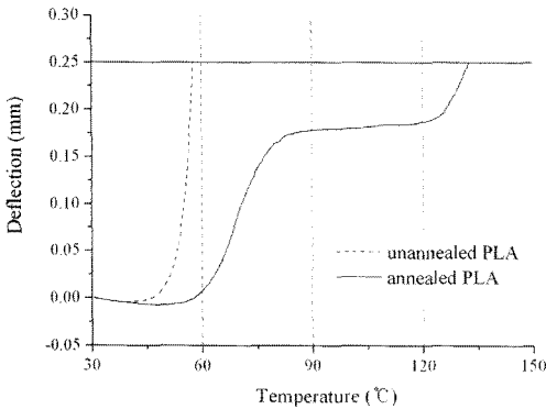
Fig. 2 Traces of HDT with a load condition of 4.6 kg/cm 2 at a heating rate of 2°C/min for unannealed PLA and PLA annealed at 120°C for 1 hr.
