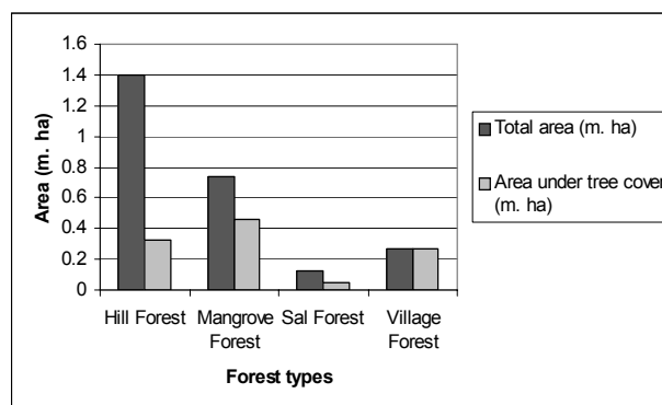
Fig. 4. Potential land available in different forest types for plantation (Adapted and modified from Roy, 2004).
