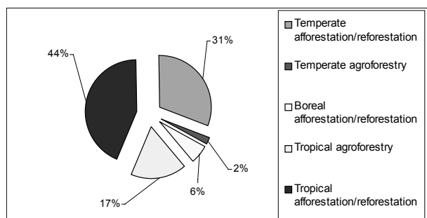
Fig. 2. Potential contribution of afforestation/reforestation and agroforestry activities to global carbon sequestration, 1995-2050 (Total carbon sequestration potential 38 gigatonnes (Gt).
