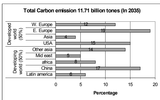
(b). Total Carbon emissions in 2035 by different countries Source: (Mintzer and Trexler, 2000).
