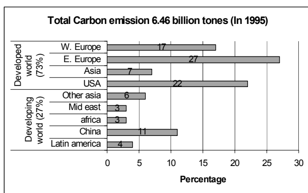
Fig. 1. (a). Total Carbon emissions in 1995 by different countries Source: (Mintzer and Trexler, 2000).
