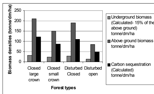
Fig. 3. Biomass densities in forest of Bangladesh (Adapted and modified from Alamgir et al., 2009).
