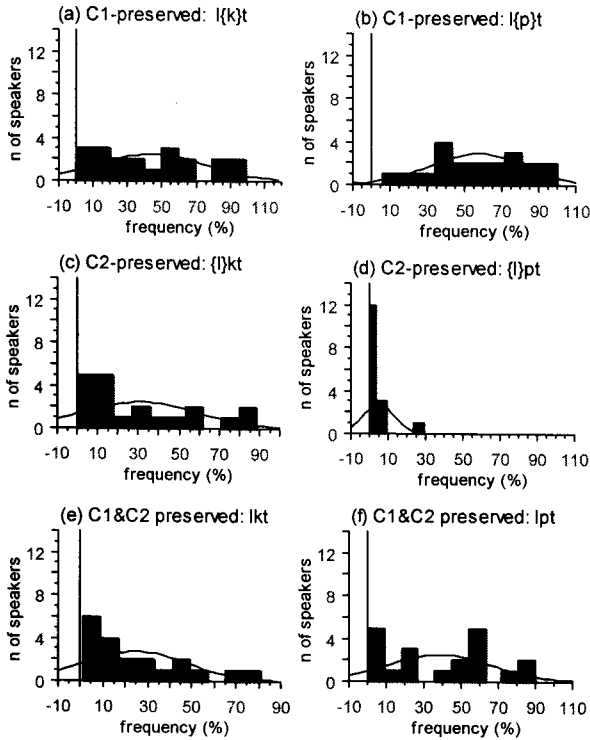
Figure 3. Inter-speaker variation of consonant cluster simplification as a function of C2 Type (/k/ vs. /p/).
