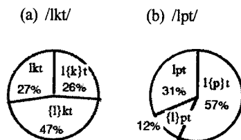
Figure 1. Frequency of three variants of tri-consonant cluster simplification for /lkt/ and /lpt/ (from Cho, 1999).
