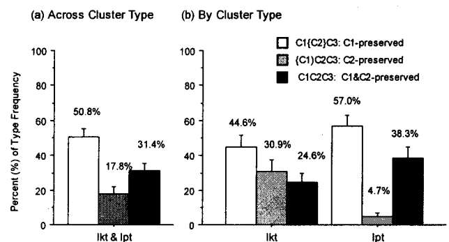
Figure 2. Overall patterns of consonant cluster simplification as a function of C2 Type (/k/ vs. /p/).
