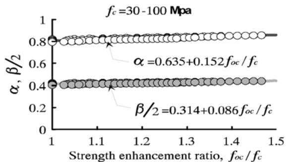
Fig. 9 Comparison of the enhancement ratio (the ratio of increase in compressive strength), f_{oc}/f_c .
