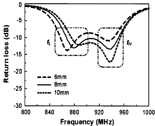
(c) 반사손실 (c) Return loss
