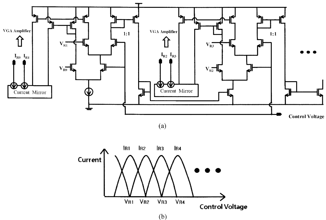
Fig. 6. The current conveyor : (a) schematic and (b) waveform of output current.
