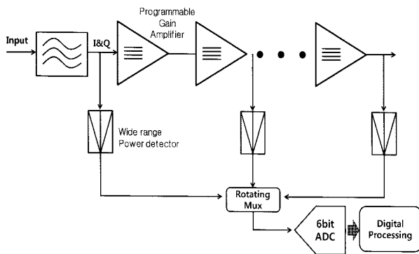
Fig. 1. Block diagram of the proposed RSSI architecture.
