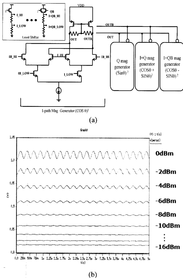
Fig. 7. Peak detector (a) structure, (b) simulation result.
