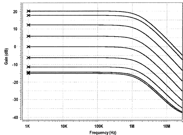
Fig. 5. AC simulation result of the proposed VGA.
