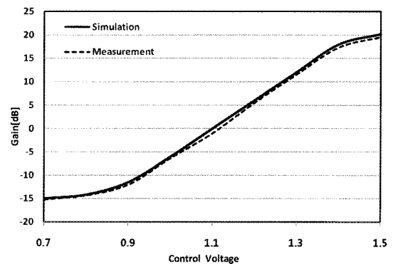
Fig. 9. Characteristic of the proposed VGA.
