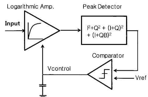
Fig. 3. Structure of the wide range power detector.
