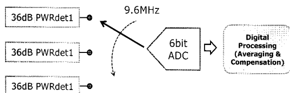
Fig. 2. Shared ADC for 3 power detectors.
