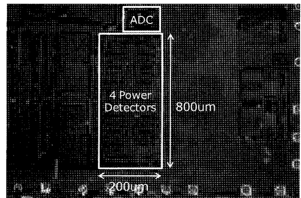
Fig. 8. Chip microphotograph.
