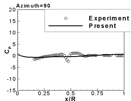
(e) Azimuth=90 deg
