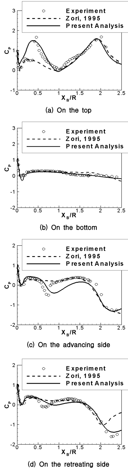
Fig. 8. Time-averaged pressure distribution on the airframe
