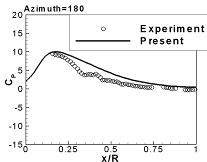
(a) Azimuth= 180 deg
