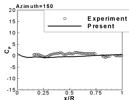
(f) Azimuth=150 deg
