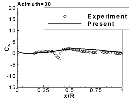
(c) Azimuth=30 deg
