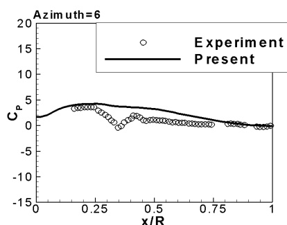
(b) Azimuth= 6 deg
