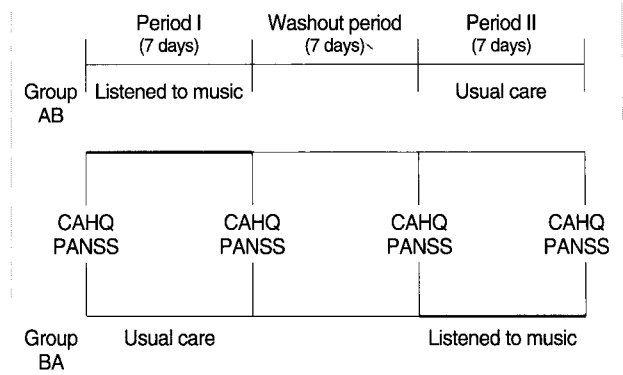
Figure 1. Research design.
