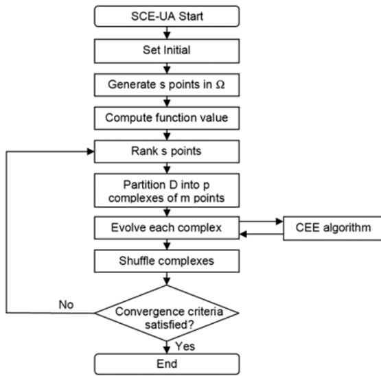
Fig. 3. Flow chart of SCE-UA algorithm(Dual et al., 1992).
