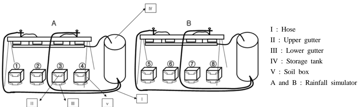
Fig. 1. Sketch of the rainfall simulator and soil-box placement.
