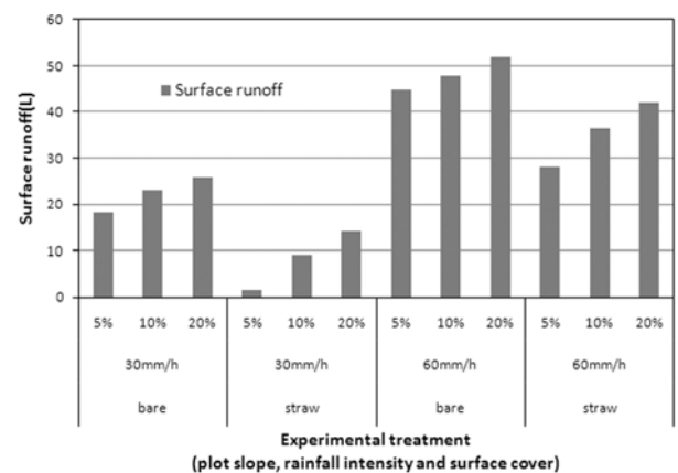
Fig. 3. Effect of experimental treatment on surface runoff with respect to slope, rainfall intensity and surface cover.
