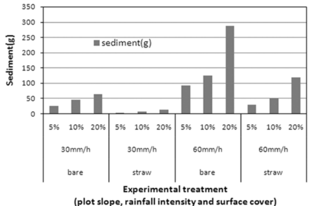
Fig. 5. Sediment affected by plot slope, rainfall intensity and landcover with respect to slope, rainfall intensity and surface cover.
