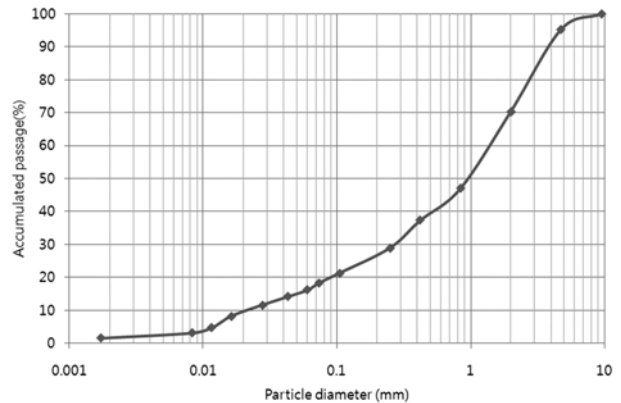
Fig. 2. Accumulated grain size distribution curve of the soil.
