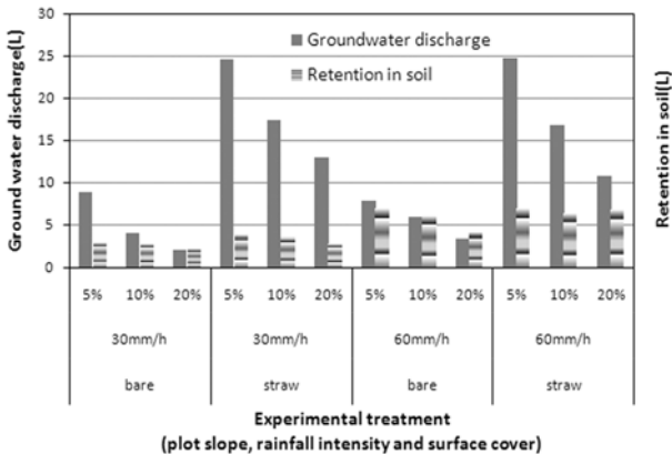
Fig. 4. Effect of experimental treatment on groundwater discharge and retention in soil with respect to slope, rainfall intensity and surface cover.
