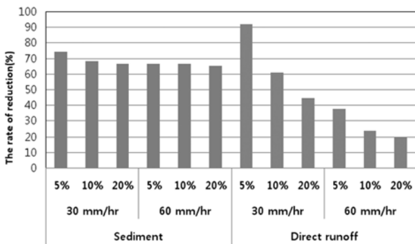
Fig. 6. The rate of reduction by plot slope, rainfall intensity and landcover with respect to slope, rainfall intensity and surface cover.
