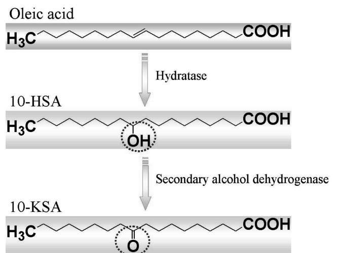
Fig. 1. Microbial conversion scheme and related enzymes for 10-KSA formation via 10-HSA from oleic acid by Flavobacterium sp. strain DS5.
