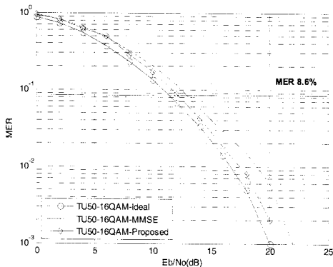
(a) Coded MER 성능(rate 1/2)
