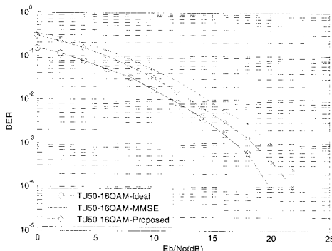
(b) Coded BER 성능(rate 1/2)
