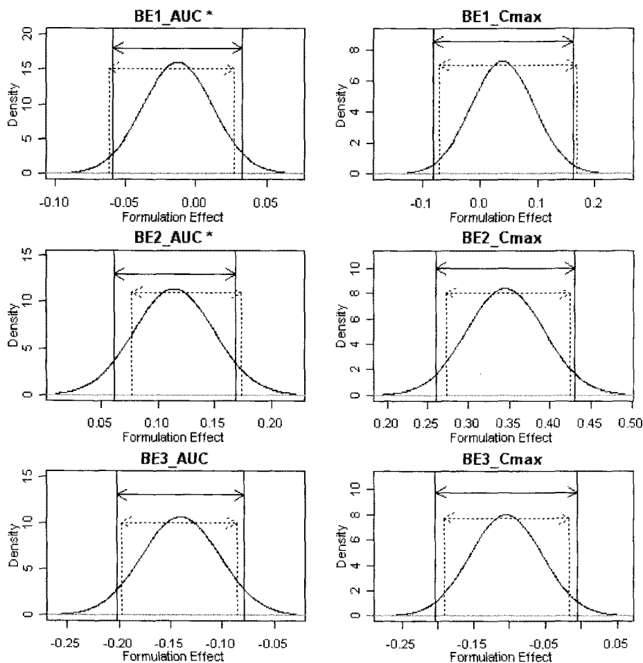
Fig. 3. Comparison of BCa 90% CIs with parametric CIs (solid lines, parametric 5% and 95% points; dotted lines, BCa 5th and 95th percentile points; density curve, anticipated parametric distribution of formulation effects from the archived datasets). *BE1_AUC and BE2_AUC were found to have non-normally distributed formulation effects by Shapro-Wilk tests.
