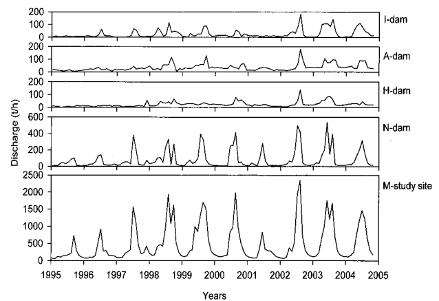
Fig. 3. Annual variation in discharge.
