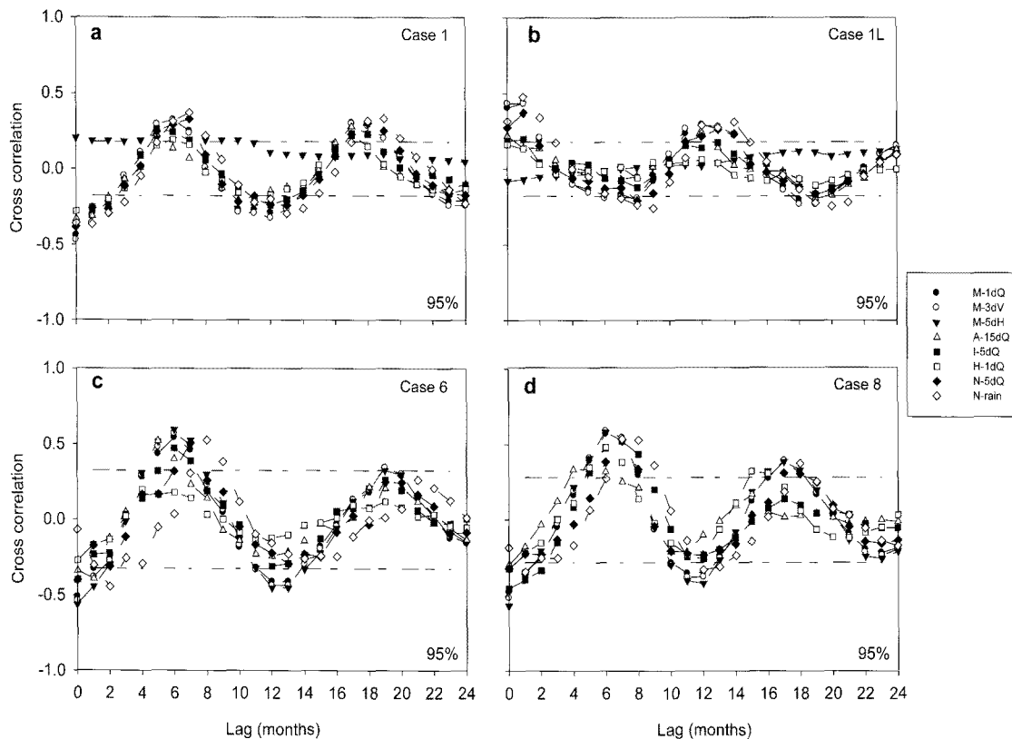
Fig. 4. Cross correlation of each factor: a (case 1)-monthly average of chl- a , b (case 1 L)-monthly average of chl- a loading, c (case 6)-monthly average of chl- a in wet years, d (case 8)-monthly average of chl- a in normal years.
