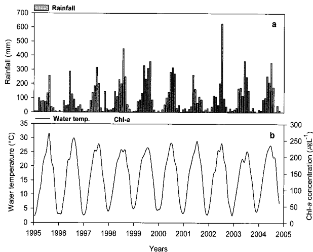
Fig. 2. Annual changes in rainfall (a), water temperature, and chl- a concentration (b) at the study site.
