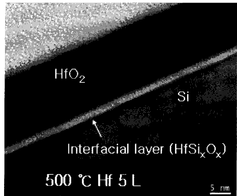
(b) \text{HfO}_2/\text{Hf}/\text{Si} structure
