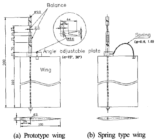
Fig. 3 Structure of the wing and shaft (unit:mm)
