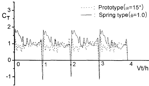
(a) Thrust coefficients
