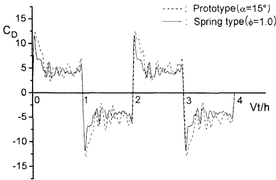
(b) Drag coefficients
