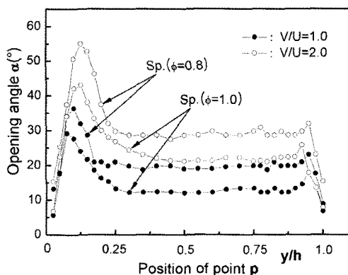
Fig. 5 Variations for opening angle according to the wing position in a stroke for each spring type elastic wing
