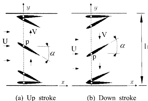
Fig. 1 A model of propulsion mechanism
