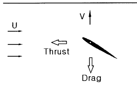
Fig. 4 Definitions of thrust and drag
