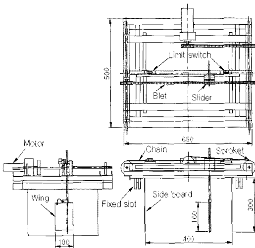
Fig. 2 Driving unit of the wing(unit:mm)
