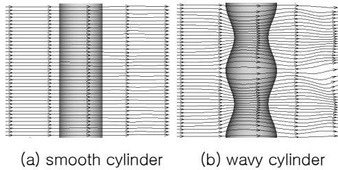
Fig. 4 Streamlines patterns
