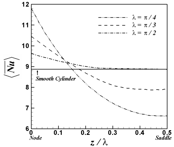
Fig. 7 Time- and spanwise local surface-averaged Nusselt number as a function of z / \lambda .
