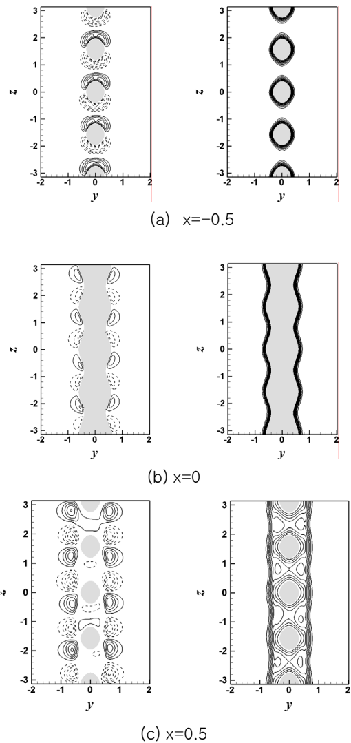
Fig. 3 Contours of the time-averaged spanwise velocity (left column) and temperature (right column) for the wavy cylinder with \lambda = \pi/2 .
