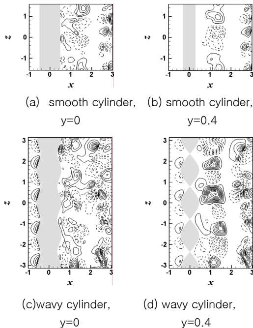
Fig. 2 Contours of instantaneous spanwise velocity in the two different x-z planes.
