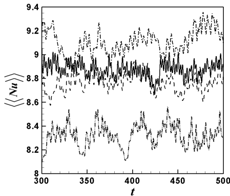
Fig. 5 Total surface-averaged Nusselt number as a function of time: \cdots , \lambda = \pi/4 ; --- , \lambda = \pi/3 ; - \cdot - , \lambda = \pi/2 ; --- , smooth cylinder.
