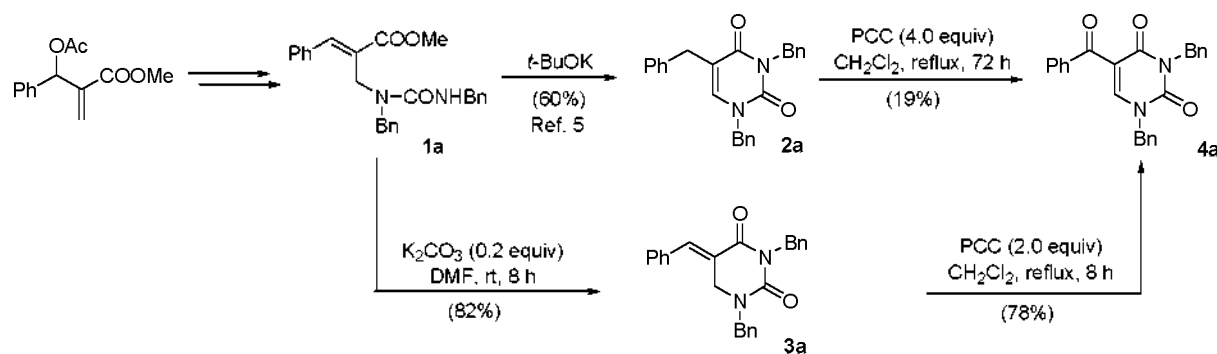
Scheme 1
