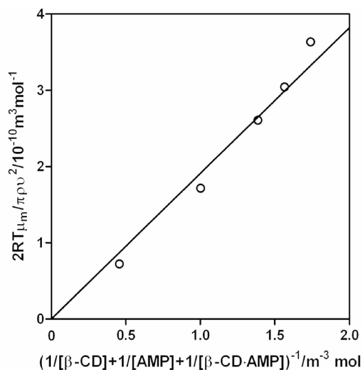
Figure 4. Plots of 2RT\mu_m/\pi\rho v^2 vs. (1/[\beta\text{-CD}] + 1/[AMP] + 1/[\beta\text{-CD} \cdot AMP])^{-1} for aqueous solution of AMP in the presence of 8.7 mM \beta -CD at 25 °C.
