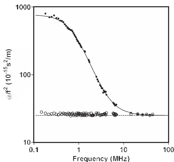
Figure 1. Ultrasonic absorption \alpha/f^2 vs. frequency in aqueous solution of AMP at 25 °C in the presence and absence of 8.7 mM \beta -CD: (○) 10mM AMP only, (●) 10 mM AMP+8.7 mM \beta -CD. The solid line represents the single relaxation curve. The dotted line represents the high-frequency limiting value (\alpha/f^2)_\infty = 25 \times 10^{-15} \text{ s}^2/\text{m} .
