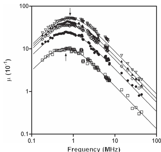
Figure 2. Excess absorption per wavelength \mu vs. frequency in aqueous solutions of AMP in the presence of 8.7mM \beta -CD at 25 °C. (□) 2mM AMP–8.7mM \beta -CD; (●) 5mM AMP–8.7mM \beta -CD; (○) 8mM AMP+8.7mM \beta -CD; (▲) 10mM AMP–8.7mM \beta -CD; (▽) 13mM AMP+8.7mM \beta -CD. The solid lines represent single relaxation curves. The arrows indicate relaxation frequencies.
