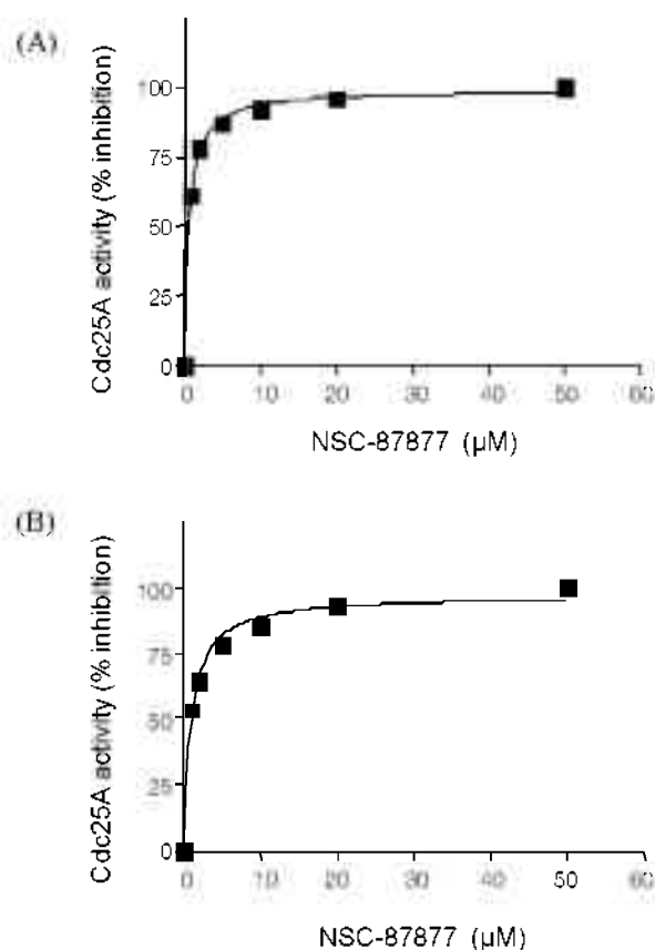
Figure 2. Inhibitory effect of NSC-87877 in Cdc25A and Cdc25B. (A) Cdc25A and was incubated with various concentrations of NSC-87877 at 37 °C for 30 min, respectively. Fluorescence emission from the product was measured with a multiwell plate reader as described in Experimental section. (B) The inhibitory effect of NSC-87877 on Cdc25B was determined as described in (A).
