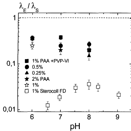
Fig. 6. Characteristic ratio \lambda_E/\lambda_S vs. pH for solutions of 1:1 mixtures of PAA and PVP-VI with PAA concentrations of 1% (■), 0.5% (●), and 0.25% (▲), pure PAA solutions at 2% (★) and 1% concentration (☆), as well as a solution of the ASE-type thickener Sterocoll FD at 1% polymer concentration (□). The dashed line indicates the typical range of \lambda_E/\lambda_S for solutions of neutral flexible polymers like poly(styrene) (Anna and McKinley, 2001) or poly(ethylenoxide) (Oliveira et al. , 2006).
