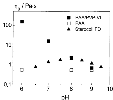
Fig. 1. Zero-shear viscosity of aqueous solutions of Sterocoll FD (▲), PAA (□) as well as 1:1 mixtures (by weight) of PAA and PVP-VI (■) as a function of pH. The concentration of the polyanion is always 1 wt.%.
