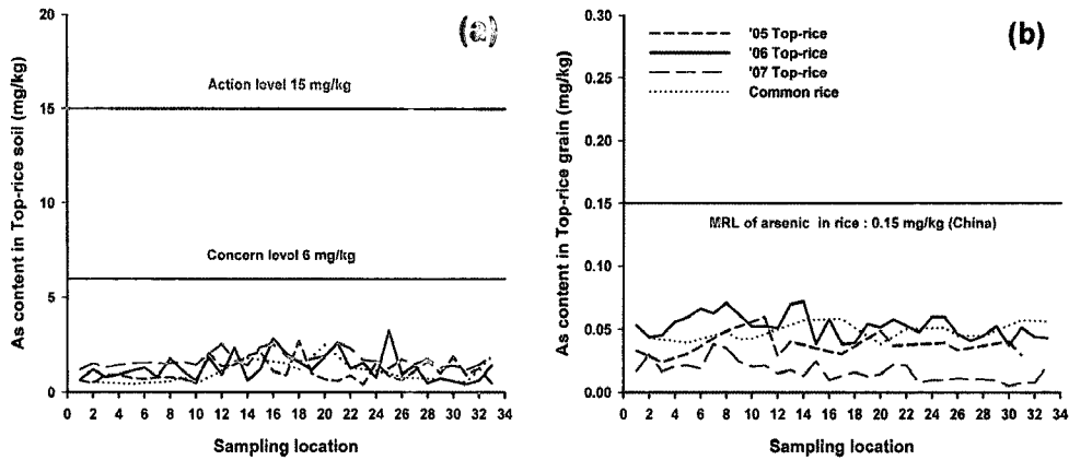
Fig. 2. Distribution of arsenic concentration in paddy soil and polished rice.
