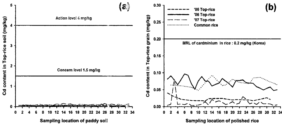
Fig. 3. Distribution of cadmium concentrations in paddy soil and polished rice.
