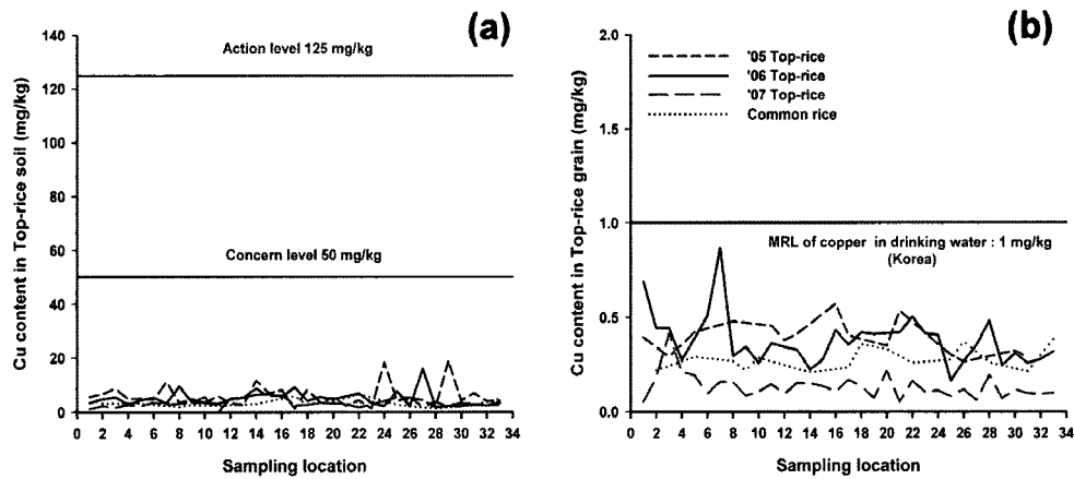
Fig. 4. Distribution of copper concentrations in paddy soil and polished rice.
