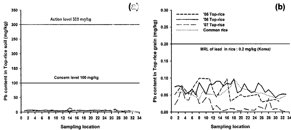
Fig. 5. Distribution of lead concentrations in paddy soil and polished rice.
