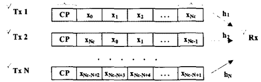
Fig. 1. The CDD scheme
