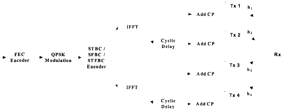
Fig. 3. Block coding technique combined with CDD
