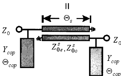
(d) A modified Π-type of transmission-line equivalent circuit with \Theta_s \leq \pi/2
