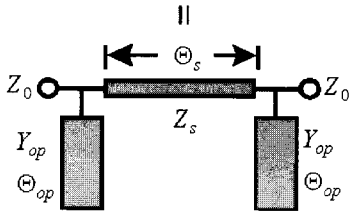
(b) A conventional Π-type of transmission-line equivalent circuit with \Theta_s \leq \pi/2
