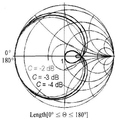
Fig. 6. Input impedances are illustrated on an impedance Smith chart depending over, critical and under coupling.
