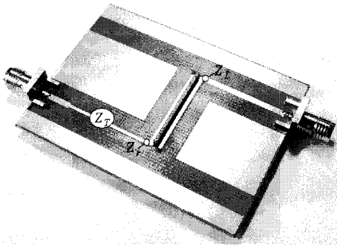
(c) Fabricated microstrip coupled lines with two shorts
