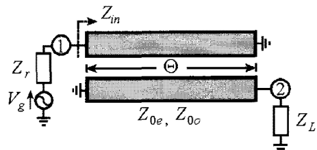
(b) Coupled-line sections with two shorts
