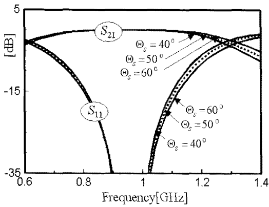
(b) Coupling C is fixed at -7 dB and \Theta_s is varied
