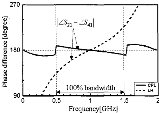
(b) Out-of-phase response
