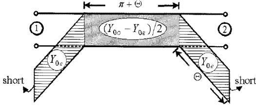
Fig. 7. Two-port equivalent circuit of coupled-line sections with two shorts.
