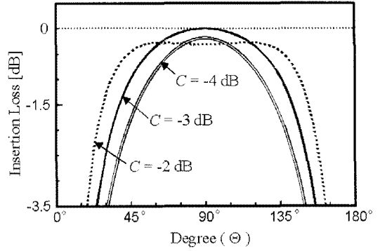
(a) Insertion loss
