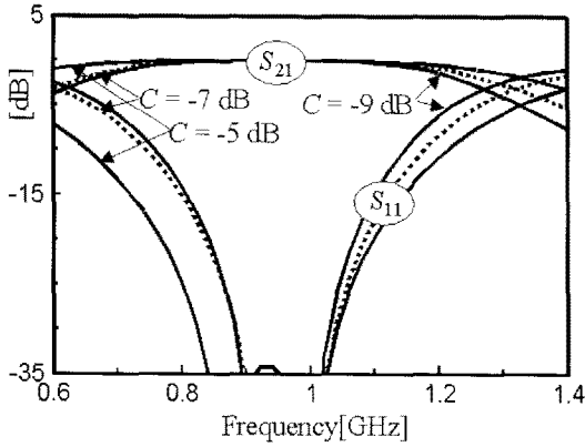
(a) \Theta_s is fixed at 60^\circ and coupling coefficients are varied
