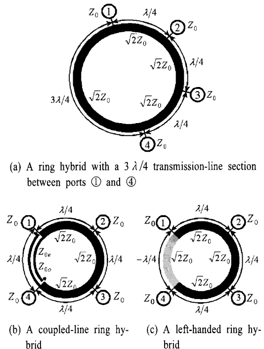
Fig. 1. Conventional ring hybrids.
