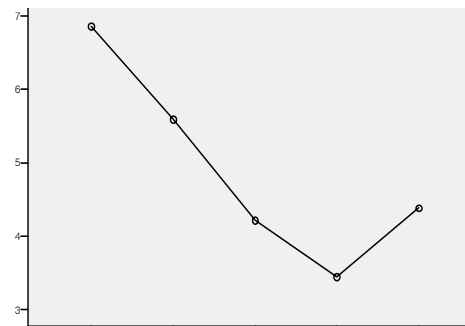
Fig. 4. Estimated marginal means of HF CONT.
