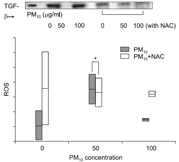
Figure 3. TGF-β expression in WI-26 VA4 cells after 24 hours incubation with PM 10 . The TGF-β levels were increased after exposed to PM 10 , compared to those in NAC and control. TGF-β expression increased after 24 hours of exposure to PM 10 in a dose-dependent manner (*p < 0.05).
