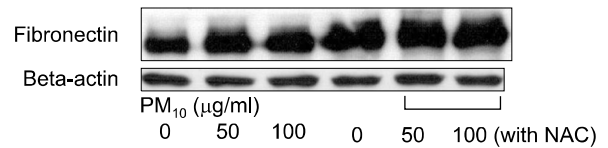
Figure 4. Fibronectin expression in WI-26 VA4 cells after 24 hours incubation with PM 10 . The fibronectin levels were increased after exposed to PM 10 , compared to those in NAC and control. fibronectin expression increased after 24 hours of exposure to PM 10 in a dose-dependent manner.
