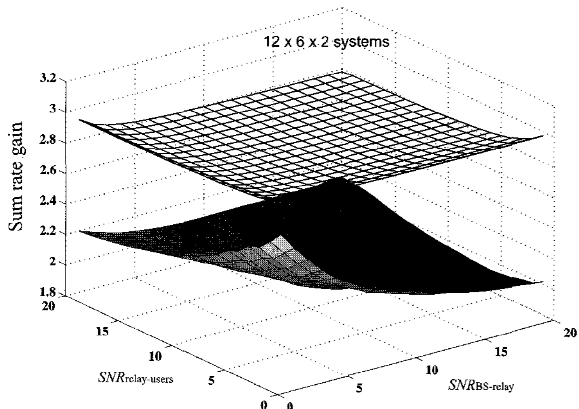
Fig. 5. Sum rate gain over TDMA strategy in \{12 \times 6 \times 2\} case.
