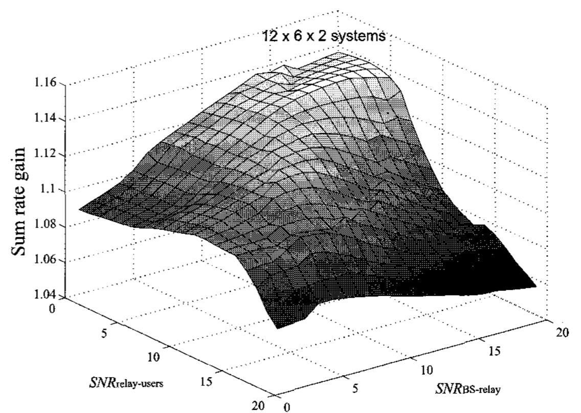
Fig. 7. Sum rate gain over BF strategy in \{12 \times 6 \times 2\} case.
