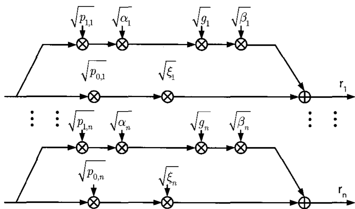
Fig. 2. Equivalent SISO relay channel.
