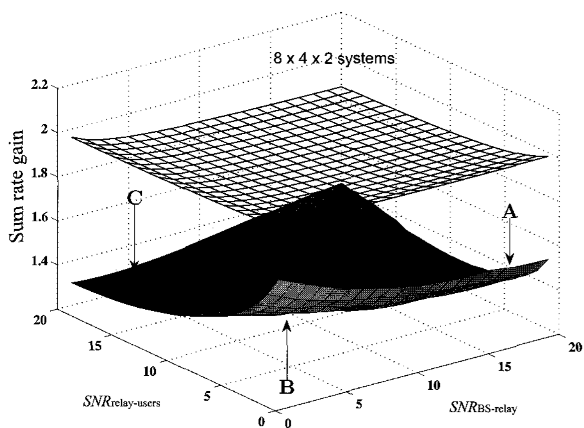
Fig. 4. Sum rate gain over TDMA strategy in \{8 \times 4 \times 2\} case.
