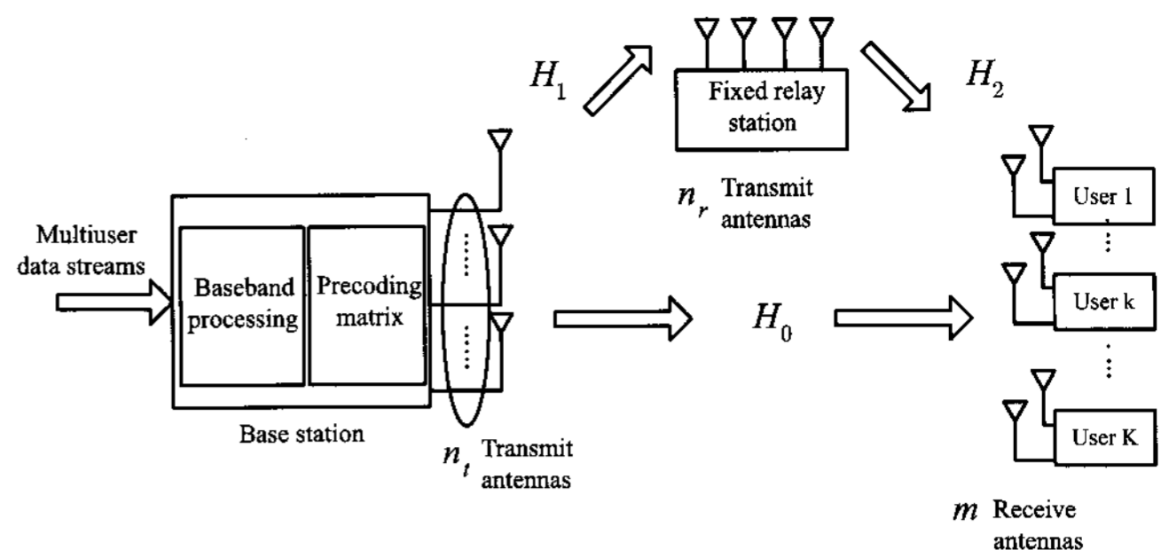
Fig. 1. System model of multiuser MIMO relay channel.
