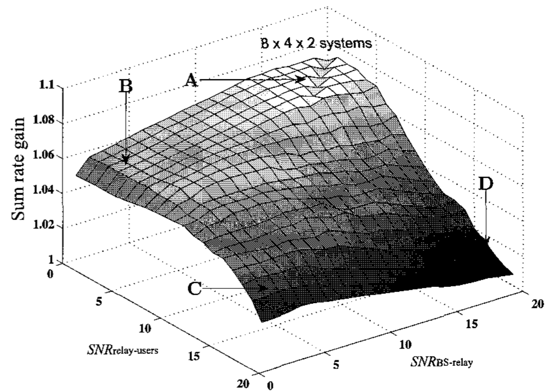
Fig. 6. Sum rate gain over BF strategy in case.
