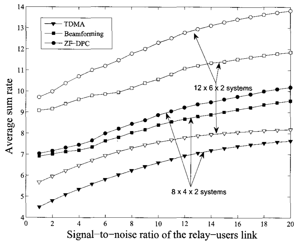
Fig. 3. Average sum rate for different BC strategies.
