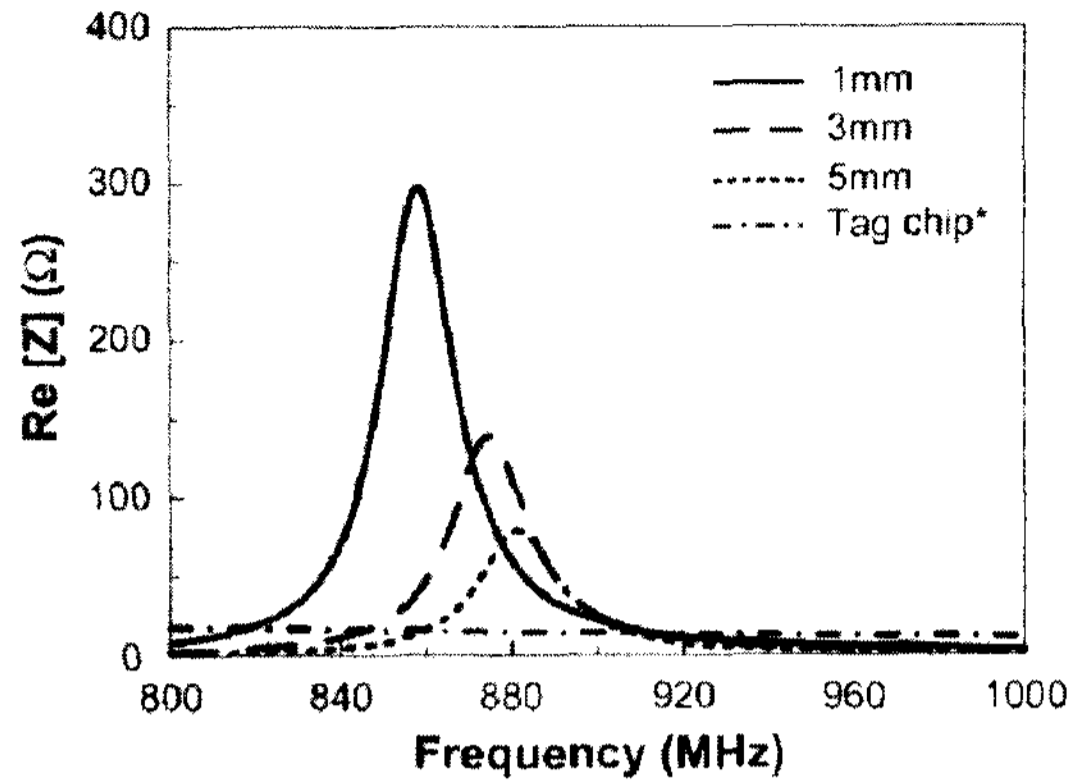
(a) 입력 저항 (a) Input resistance
