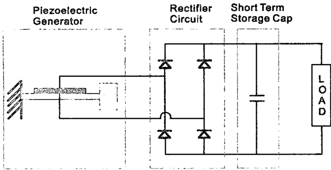
Fig. 4 Electrical circuit for piezoelectric energy harvesting system
