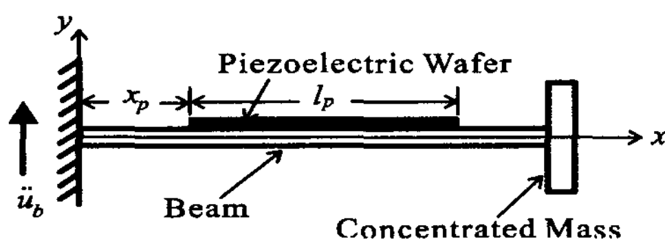
Fig. 1 Schematics of cantilever-type piezoelectric energy harvesting device with a tip mass
