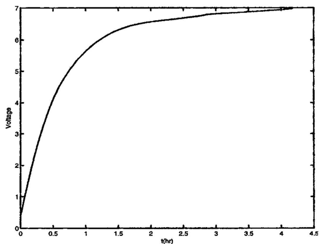
Fig. 9 Voltage charging for the 0.1F super capacitor
