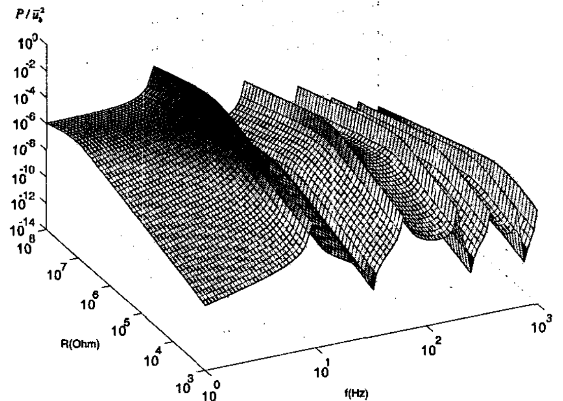
Fig. 3 Power curve vs. frequency and resistance
