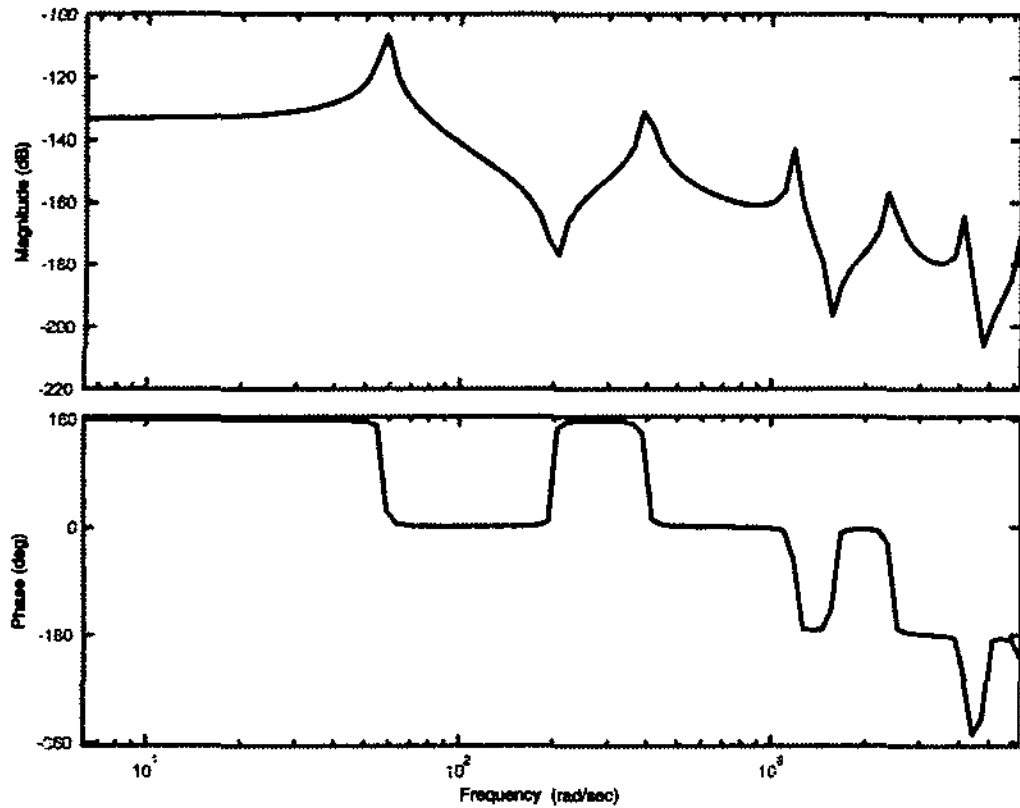
Fig. 2 Transfer function of energy harvesting device
