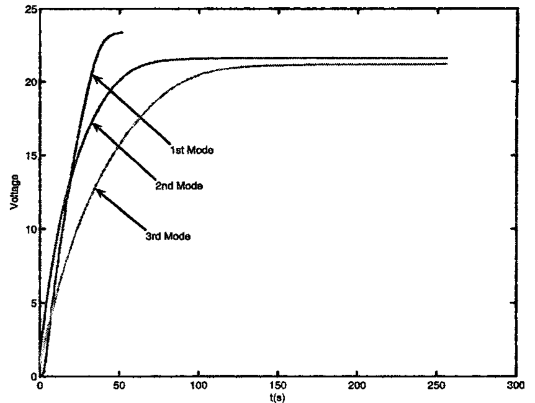
Fig. 7 Voltage charging for the 220 \mu\text{F} capacitor
