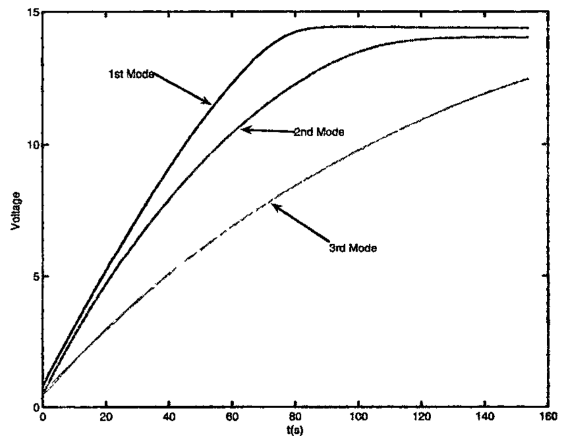
Fig. 8 Voltage charging for the 1000 \mu\text{F} capacitor
