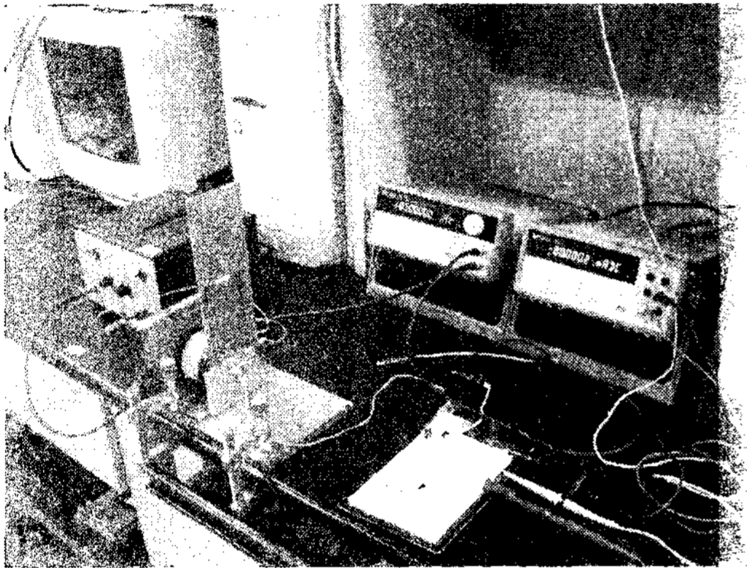
Fig. 5 Experimental setup for piezoelectric energy harvesting system
