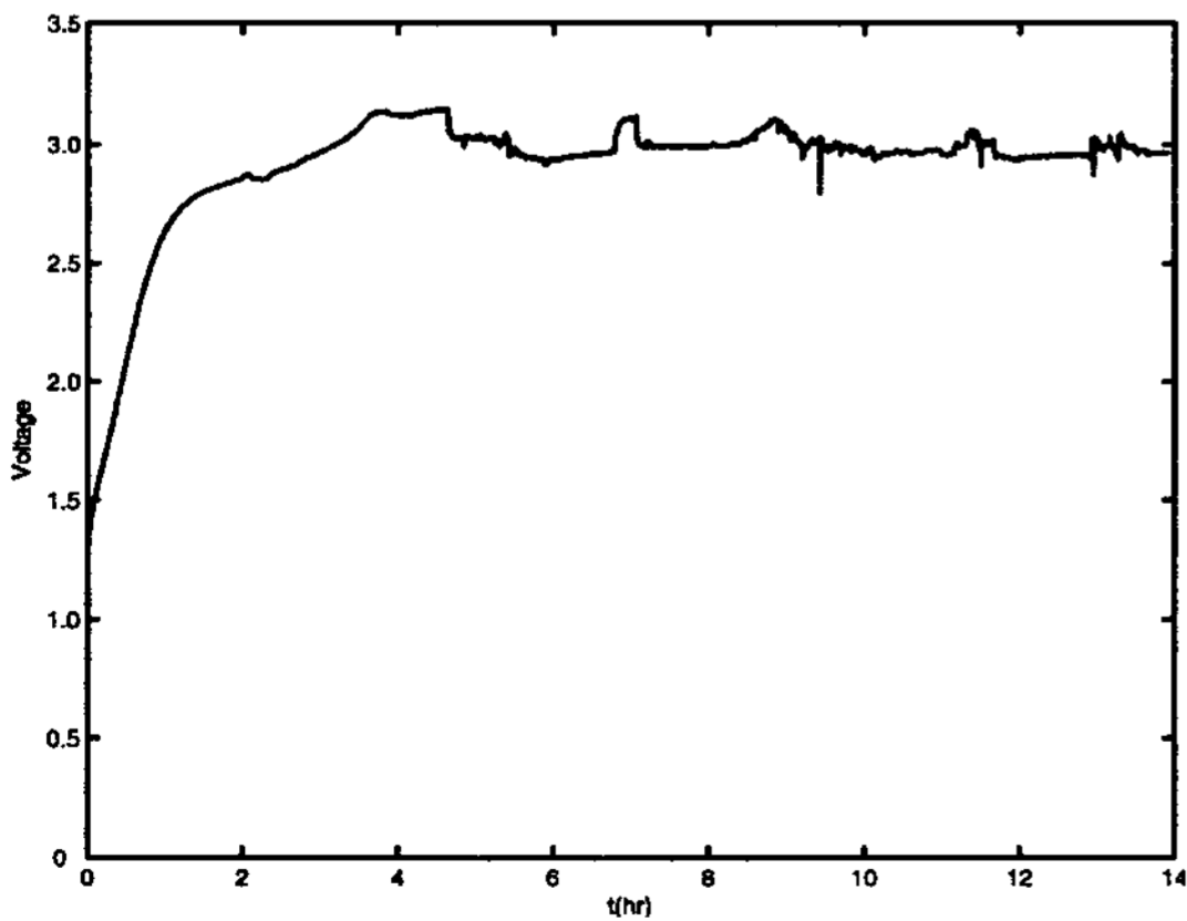
Fig. 10 Voltage charging for the 0.1F super capacitor (44)
