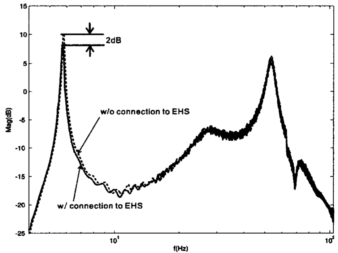
Fig. 12 Change in frequency response curve by the introduction of the energy harvesting system (44)
