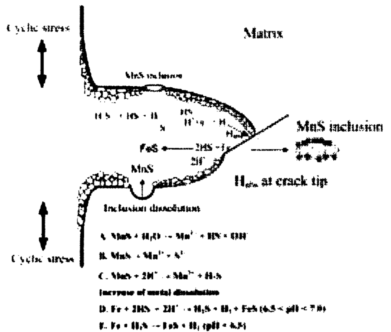
Fig. 7. Schematic Illustration of the Role of MnS Inclusions
