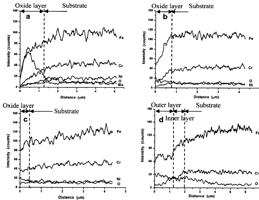
Fig. 6. EDS Line-Scan Profiles Over a Cross-Section of Stainless Steels Samples Tested After 500 h: (a) 316L, (b) 304, (c) N Controlled 304L, and (d) 410
