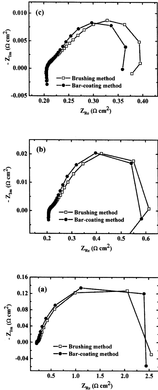
Fig. 8. Nyquist plots of single cells at (a) 0.3 V, (b) 0.4 V and (c) 0.5 V (Anode/cathod : 1.5 M methanol fuel/Hydrogen).
