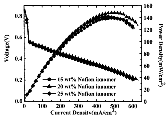
Fig. 5. Polarization curves of the MEAs with different Nafion ionomer contents in cathode catalyst layer.
