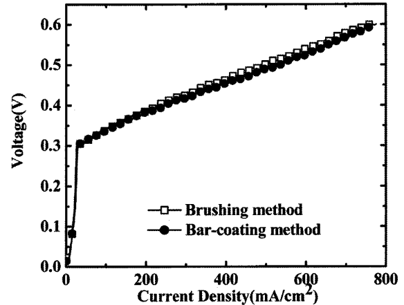
Fig. 7. Anode polarization curves of MEAs prepared by brushing and by bar-coating methods (cell temperature: 60 °C) (Anode/cathode : 1.5 M methanol fuel/Hydrogen).
