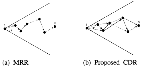
Fig. 1 Routing strategies
