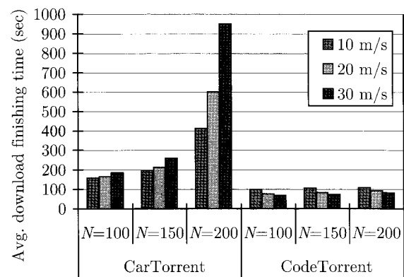
Fig. 4. Impact of mobility on average download delay.
