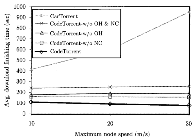
Fig. 7. Comparison of CodeTorrent and its variants ( N = 200 , 40% popularity).
