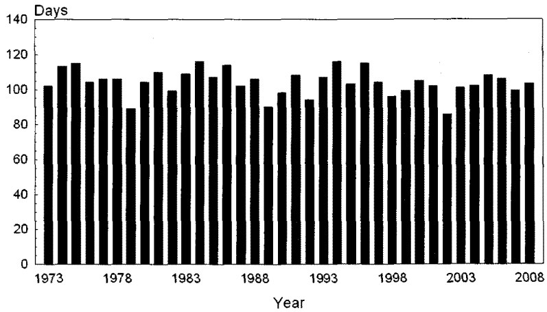
Figure 7. Change in the frequency of days below -3°C minimum temperature (December-March)
