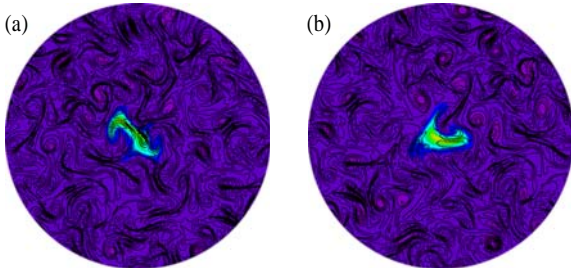
Fig. 11 Distributions of temperature and vorticity in induction phase for HR71-1 (a) and HR71-2 (b) ( t/\tau_f=0.412 )
