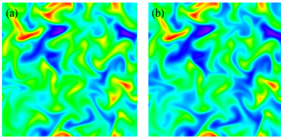
Fig. 15 Temperature distribution in the auto-ignition process of inhomogeneous mixture ( \phi'=0.2 ) for Re_\lambda=106 , T_{ini}=1750\text{K} and P_{ini}=0.2\text{MPa} . (a): t=82\mu\text{s} , temperature range[1879.44, 1941.26(K)] and (b): t=86\mu\text{s} , temperature range[1970.46, 2158.99(K)]
