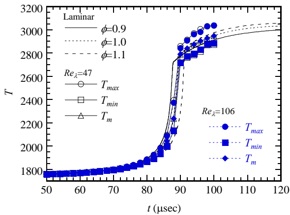
Fig. 16 Effects of Reynolds number on temperature developments for inhomogeneous mixture ( \phi=0.1 ) for T_{mi}=1750\text{K} and P_{mi}=0.2\text{MPa}
