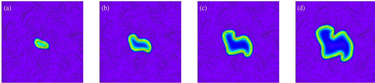
Fig. 7 Temporal developments of distributions of heat release rate and vorticity in propagation process for HR47 ((a) t/\tau_f=0.74 , (b) t/\tau_f=1.07 , (c) t/\tau_f=1.40 , (d) t/\tau_f=1.73 )
