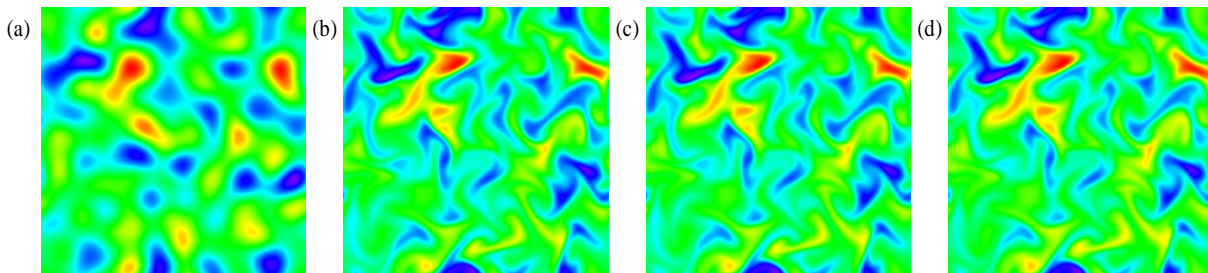
Fig. 14 Development of mole fraction of \text{CH}_4 in the auto-ignition process of inhomogeneous mixture ( \phi'=0.2 ) for Re_\lambda=106 , T_{ini}=1750\text{K} and P_{ini}=0.2\text{MPa} . (a): t=0 , mole fraction range[0.079, 0.11], (b): t=82\mu\text{s} , mole fraction range[0.049, 0.082], (c): t=84\mu\text{s} , mole fraction range[0.04, 0.077], and (d): t=86\mu\text{s} , mole fraction range[0.026, 0.07]
