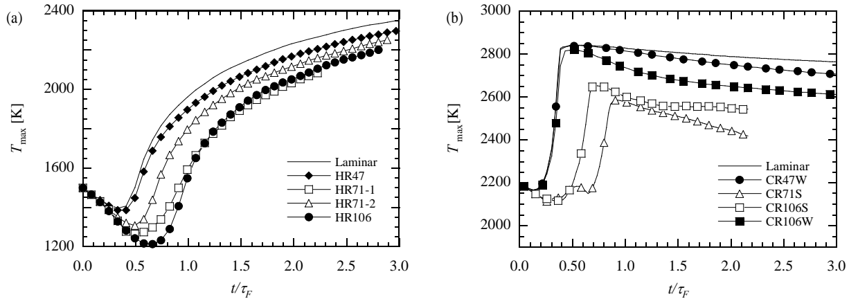
Fig. 6 Temporal developments of maximum temperature for hydrogen/air cases (a) (Laminar, HR47, HR71-1, HR71-2 and HR106) and methane/air cases (b) (Laminar, CR47W, CR71S, CR106S and CR106W)
