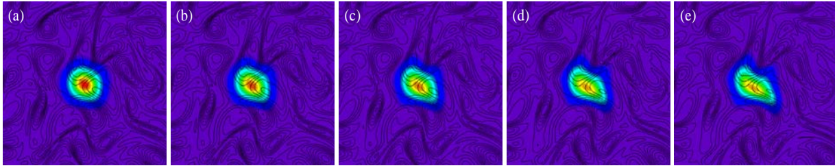
Fig. 3 Temporal developments of temperature and vorticity in induction phase for HR47 ((a) t/\tau_f=0.0825 , (b) t/\tau_f=0.165 , (c) t/\tau_f=0.247 , (d) t/\tau_f=0.330 , (e) t/\tau_f=0.412 )
