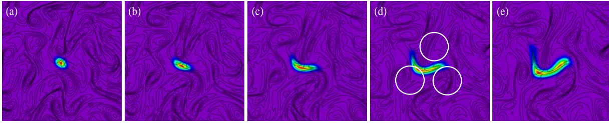
Fig. 5 Temporal developments of mole fraction of H atom with vorticity distribution in induction phase for HR106 ((a) t/\tau_F=0.0825 , (b) t/\tau_F=0.247 , (c) t/\tau_F=0.412 , (d) t/\tau_F=0.742 , (e) t/\tau_F=0.825 )
