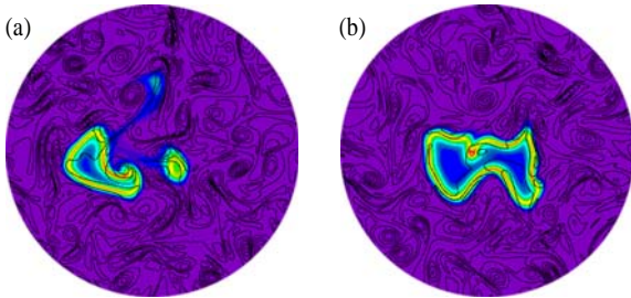
Fig. 12 Distributions of heat release rate and vorticity in propagation process for HR71-1 (a) and HR71-2 (b) ( t/\tau_f=1.40 )
