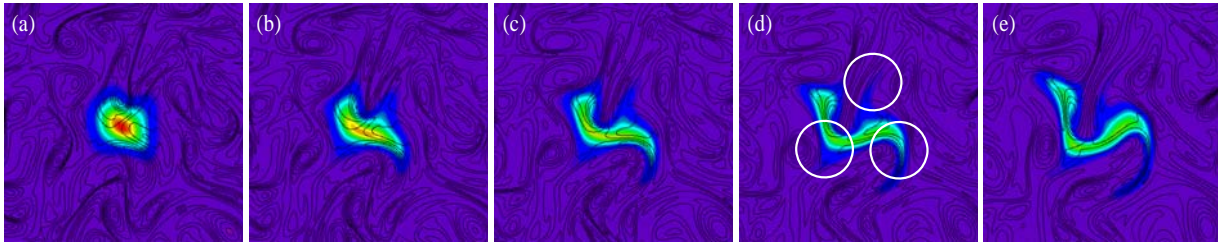
Fig. 4 Temporal developments of temperature and vorticity in induction phase for HR106 ((a) t/\tau_f=0.0825 , (b) t/\tau_f=0.247 , (c) t/\tau_f=0.412 , (d) t/\tau_f=0.742 , (e) t/\tau_f=0.825 )
