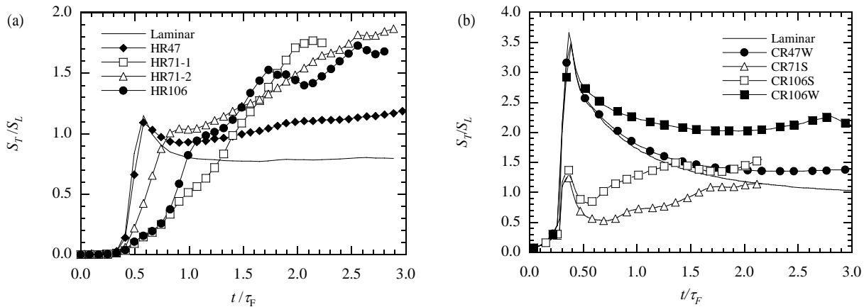
Fig. 9 Temporal developments of the turbulent burning velocity for hydrogen/air cases (Laminar, HR47, HR71-1, HR71-2 and HR106) and methane/air cases (Laminar, CR47W, CR71S, CR106S and CR106W)
