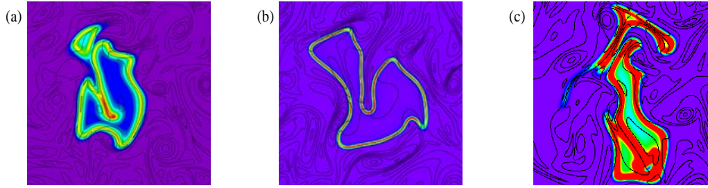
Fig. 10 Distributions of heat release rate and vorticity in propagation process for HR106 (a), CR106W (b) and C7R106 (c) ((a) t/\tau_f=1.73 , (b) t/\tau_f=1.95 , (c) t/\tau_f=1.85 )
