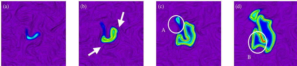
Fig. 8 Temporal developments of distributions of heat release rate and vorticity in propagation process for HR106 ((a) t/\tau_f=0.74 , (b) t/\tau_f=1.07 , (c) t/\tau_f=1.40 , (d) t/\tau_f=1.73 )
