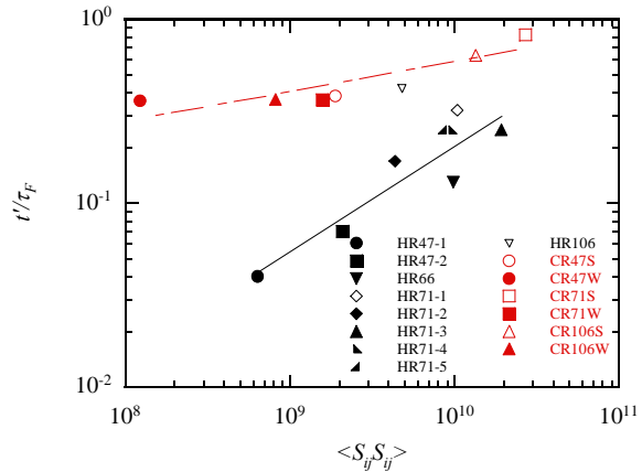
Fig. 13 Relation between ignition delay and mean strain rate
