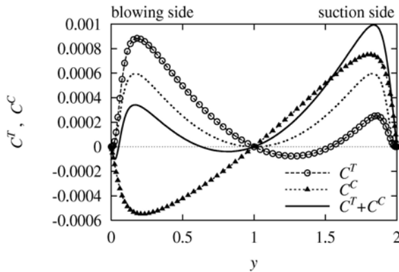
Fig. 5 Contributions to friction drag in channel flow at Re_{\tau 0} = 180 with uniform blowing and suction[8]
