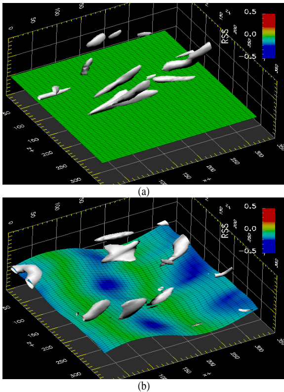
Fig. 13 Motion of the wall, Reynolds shear stress on the wall (color), and the vortical structure (white): (a) solid wall (b) anisotropic compliant surface[32]
