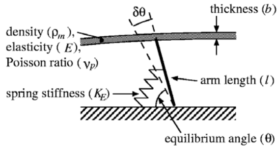
Fig. 12 Anisotropic compliant surface model[32,33]
