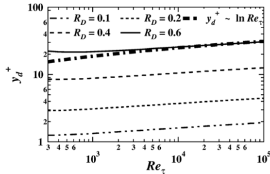
Fig. 7 Thickness of the damping layer, y_D^+ , required to achieve the same drag reduction rate, Re_D [23]
