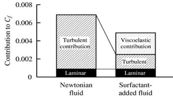
Fig. 6 Contributions to friction drag in surfactant-added channel flow. Redrawn based on Yu et al.[12]
