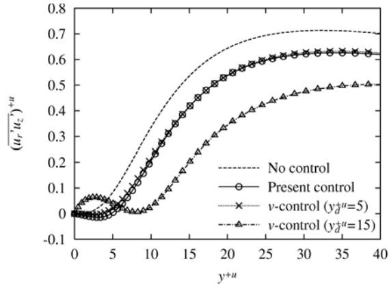
Fig. 10 Reynolds shear stress in pipe flow at Re_\tau = 180 under the Reynolds shear stress-based suboptimal control[25]
