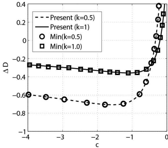
Fig. 11 Drag increment \Delta D as functions of wavespeed c and wavenumber k in of Min et al.'s traveling wave control[29] reproduced by Mamori et al.[30]
