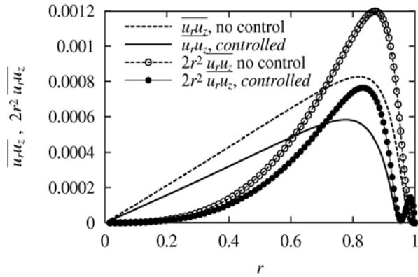
Fig. 3 Reynolds shear stress and weighted Reynolds shear stress in pipe flow at Re_{\tau 0} = 180 under opposition control[8]
