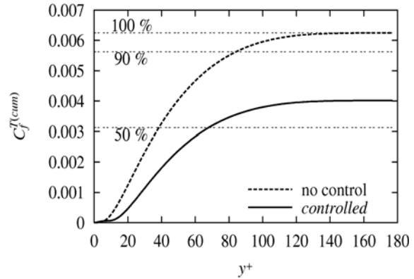
Fig. 4 Cumulative contribution to skin friction in pipe flow at Re_{\tau 0} = 180 under opposition control[8]
