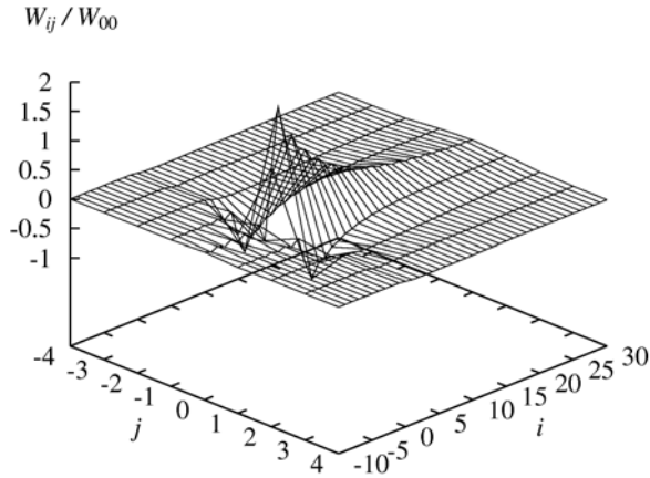
Fig. 9 Weight distributions of the Reynolds shear stress-based suboptimal control law[25]
