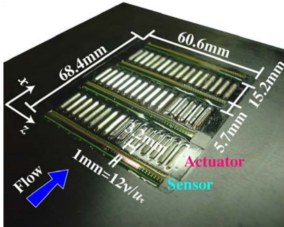
Fig. 1 Feedback control system for wall turbulence with 192 MEMS wall-shear-stress sensors and 48 magnetic shell-deformation actuators developed by Yoshino et al. [2]
