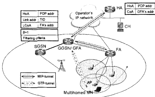
Fig. 4. Change of visitor list entry at GFA after MIP-RR registration.
