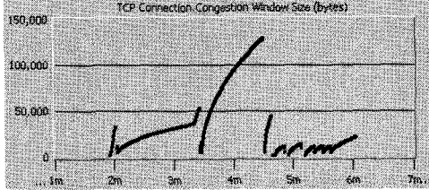
(b) Congestion window of FTP server.
