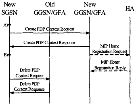
Fig. 5. Inter-GGSN/GFA handover signaling in the stage II.
