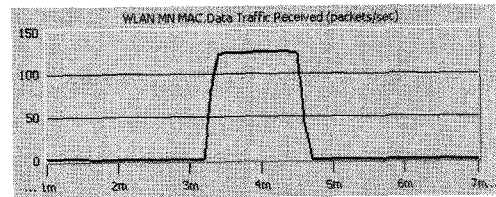
(d) Traffic received by MN from WLAN.
