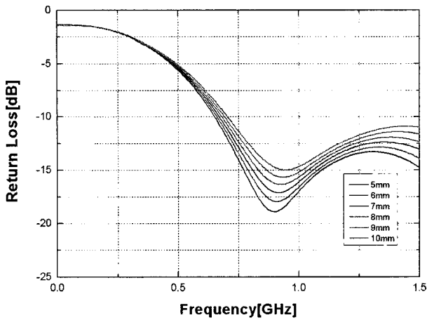
Fig. 2 L_9 optimization as to S_{11} from 5mm to 10mm
