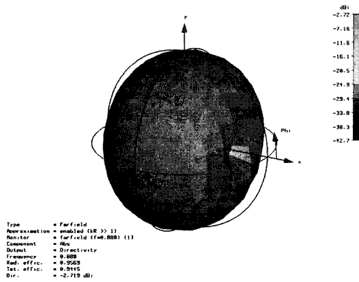
Fig. 7 Simulated far-field radiation pattern.
