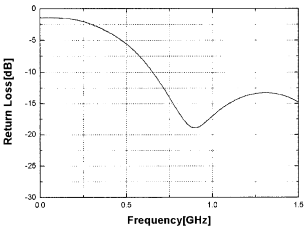
Fig. 4 Return loss simulation results with final dimensions showing -10dB bandwidth.
