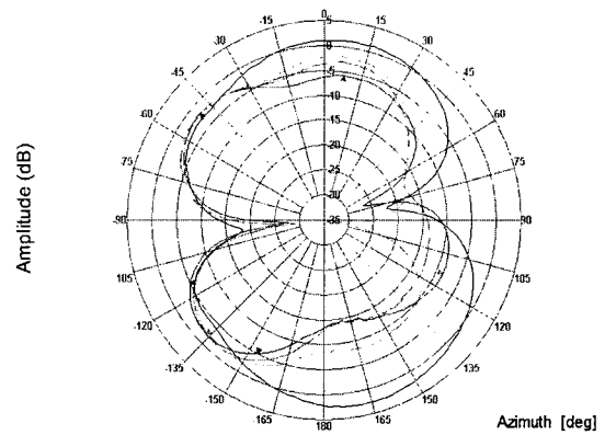
Fig. 10 Measured E-pattern at 910MHz.
