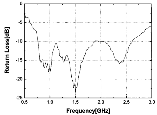
Fig. 9 Measured return loss for the proposed antenna
