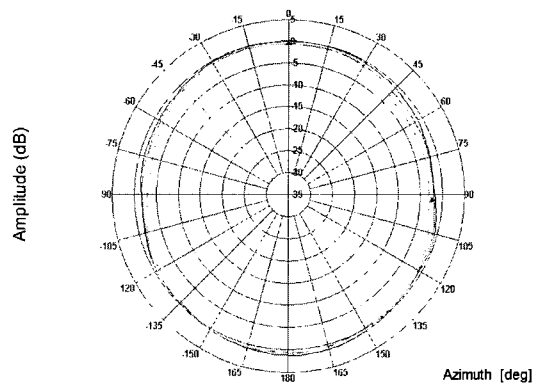
Fig. 11 Measured H-pattern at 910MHz.
