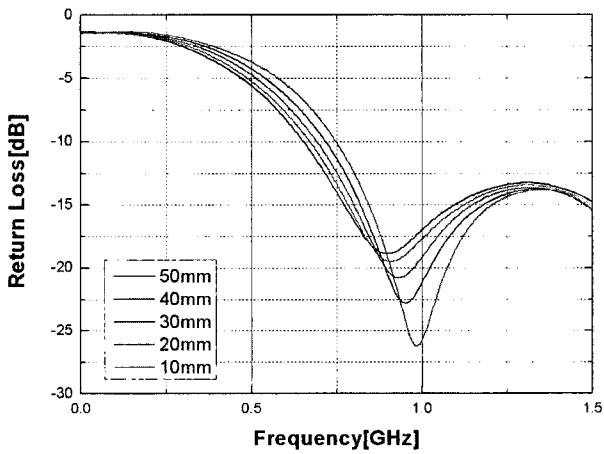
Fig. 3 L_2 optimization as to S_{11} from 10mm to 50mm
