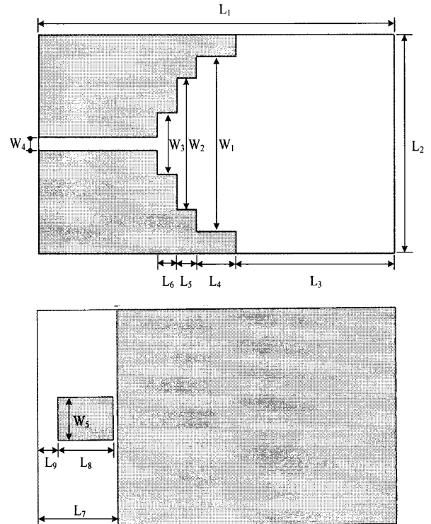
Fig. 1 Geometry of the proposed RFID antenna.
