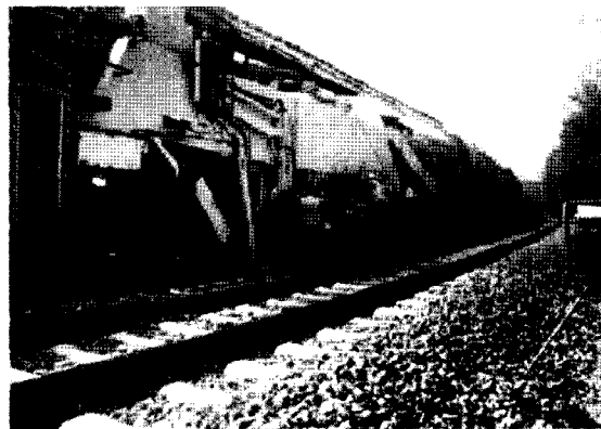
Fig. 2 Working Gang with Heavy Construction Machine on a Two-track Line while the Traffic Regularly Goes on [2]
