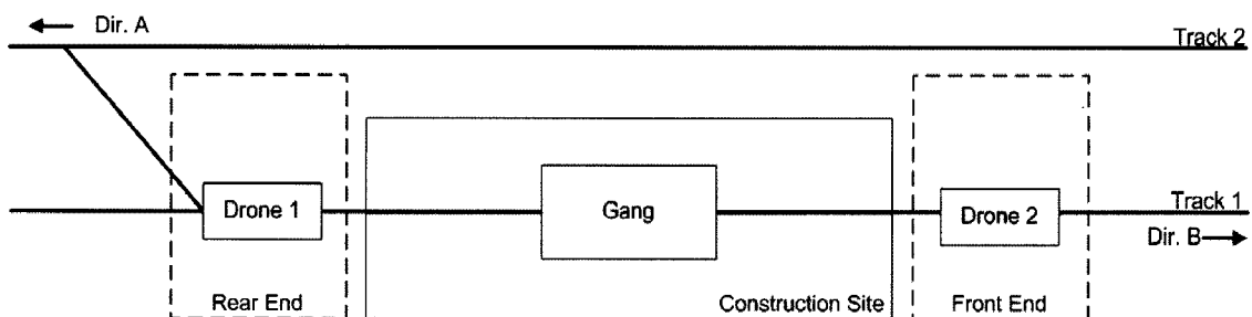
Fig. 7 Parts of the Construction Site for the Equipment with the Protection System
