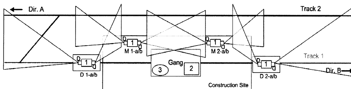
Fig. 9 Example construction site with equipment and the angel of view of the cameras
