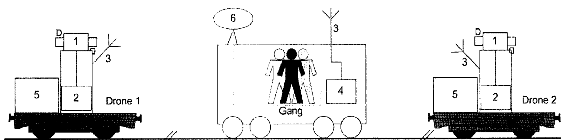
Fig. 5 System Architecture of the Gang Protection System
