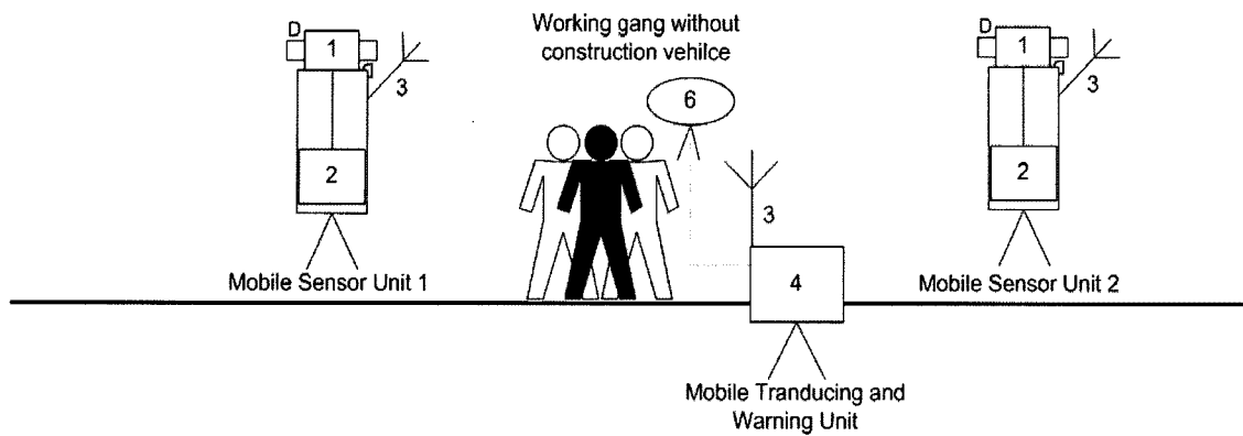
Fig. 6 System Architecture of the Gang Protection System in a Schematic View
