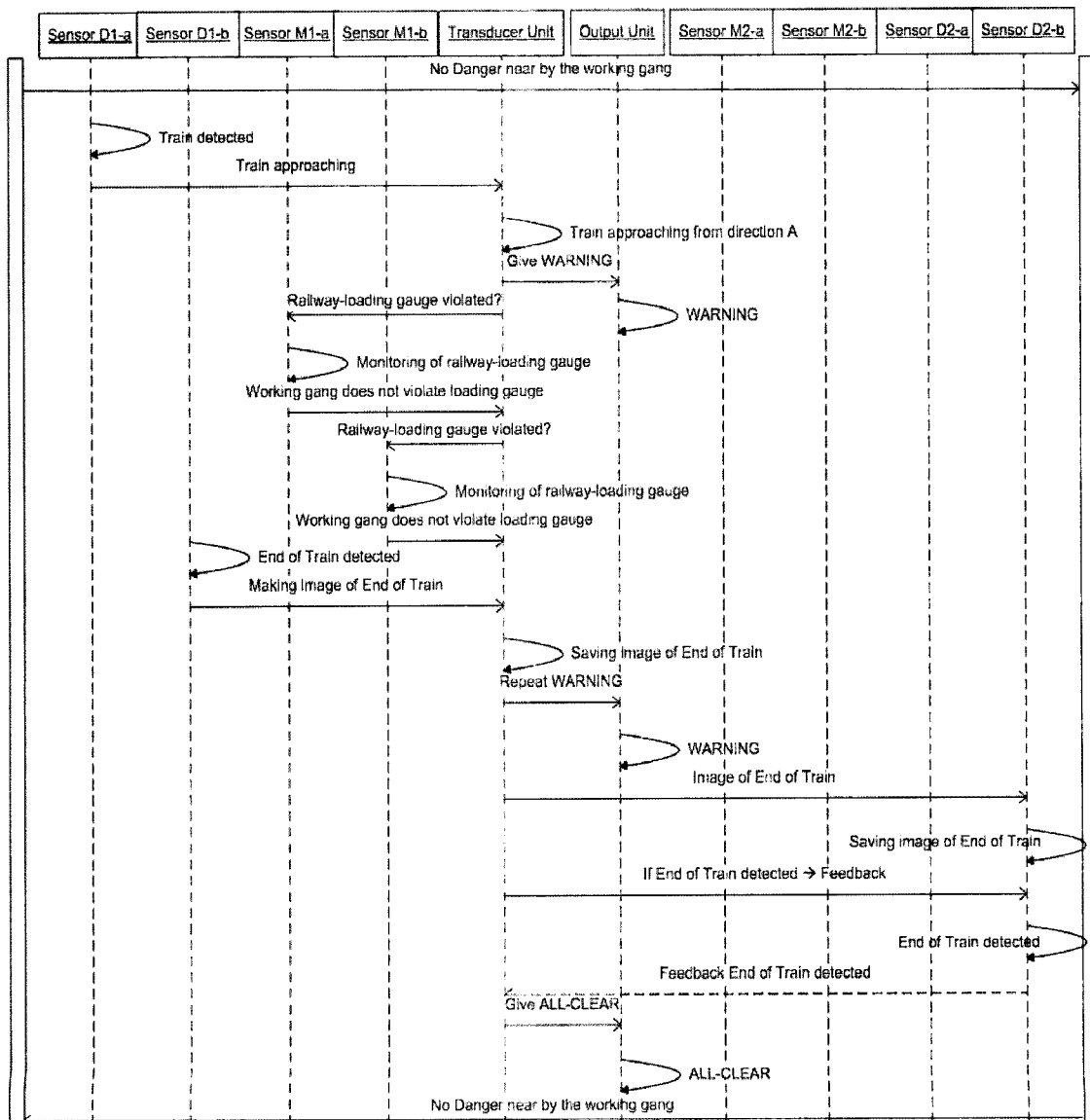
Fig. 11 Actions of the protection system during gang warning
