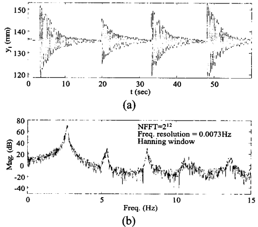
Fig. 6 Dynamic responses of test No.2: (a) displacement; (b) cross spectrum
