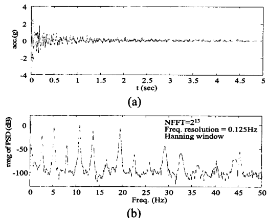
Fig. 7 Dynamic responses of test No.3: (a) acceleration (b) cross spectrum
