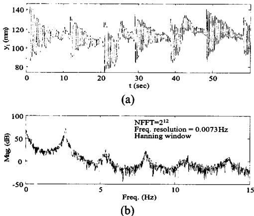
Fig. 5 Dynamic responses of test No.1: (a) displacement; (b) cross spectrum
