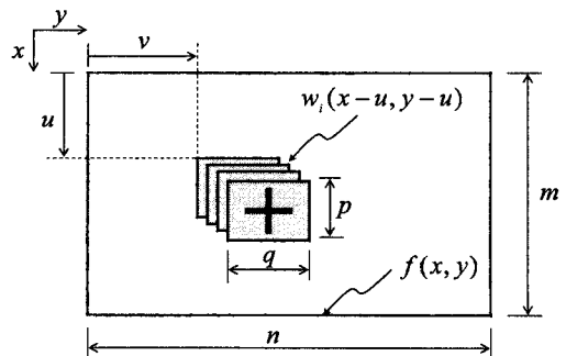
Fig. 2 Multiple template matching process
