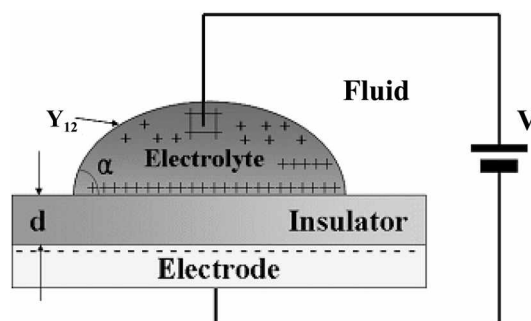
Figure 3. Electro-wetting properties in the liquid lens.
