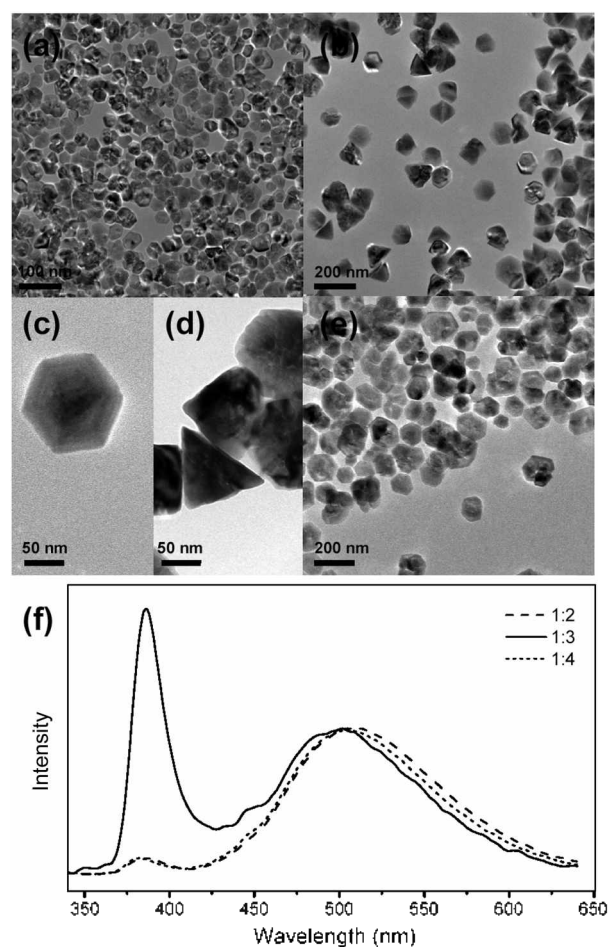
Figure 1. (a) The TEM image of ZnO nanoparticles prepared by Method I (ZnAc 2 :TOPO = 1:2). (b) The TEM image of ZnO nanoparticles prepared by Method I (ZnAc 2 :TOPO = 1:3). (c) (top view) The magnified TEM image presents a hexagonal shape of ZnO nanoparticle (ZnAc 2 :TOPO = 1:3). (d) (side view) The magnified TEM image presents a cone shape of ZnO nanoparticle (ZnAc 2 :TOPO = 1:3). (e) The TEM image of ZnO nanoparticles prepared by Method I (ZnAc 2 :TOPO = 1:4). (f) Photoluminescence spectra of ZnO nanoparticles prepared by Method I. The molar ratios of TOPO to ZnAc 2 are presented in the inset, i.e. , ZnAc 2 :TOPO = 1:2, 1:3, and 1:4.
