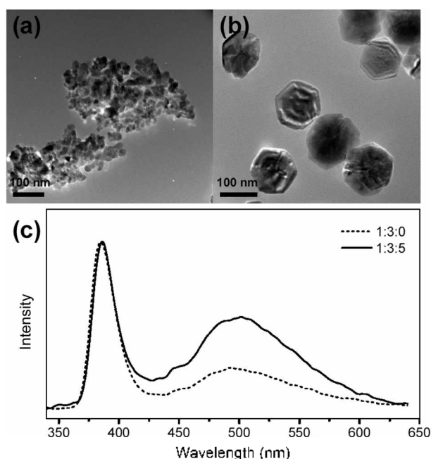
Figure 2. (a) The TEM image of ZnO nanoparticles prepared by Method I without OA ( \text{ZnAc}_2 :TOPO:OA = 1:3:0). (b) The TEM image of ZnO nanoparticles prepared by Method I with OA ( \text{ZnAc}_2 :TOPO:OA = 1:3:5). (c) Photoluminescence spectra of ZnO nanoparticles prepared by Method I by changing the molar ratio of OA. The molar ratios of OA to \text{ZnAc}_2 and TOPO are presented.
