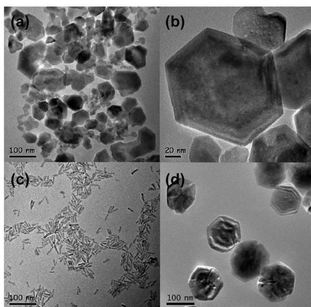
Figure 3. (a) The TEM image presents the hexagonal plate shapes of ZnO nanoparticles prepared by Method II. (b) The magnified TEM image (Method II) presents a clear view of the hexagonal shapes of ZnO nanoparticles. (c) The TEM image presents the nanorod shapes of ZnO nanoparticles prepared by Method III. (d) The TEM image presents the hexagonal cone shapes of ZnO nanoparticles prepared by Method I.
