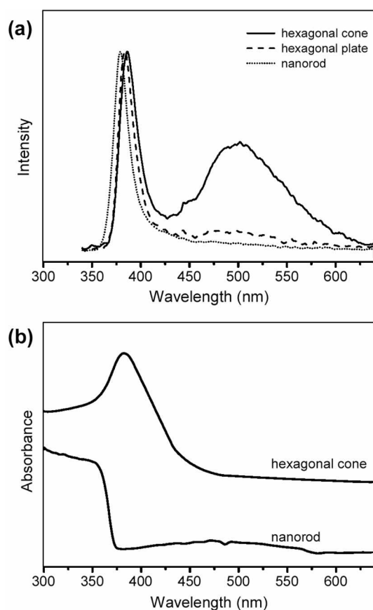
Figure 4. (a) Photoluminescence spectra of the ZnO nanoparticles prepared by Method I, II, and III. The hexagonal cone, hexagonal plate, and nanorod are prepared by Method I, II, and III, respectively. (b) Absorption spectra of the ZnO nanoparticles prepared by Method I and III. The hexagonal cone and nanorod are prepared by Method I and III, respectively.
