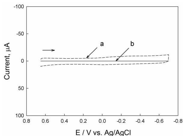
Figure 2. Cyclic voltammograms in pure supporting electrolyte at the EPG electrode (a) without (dashed) and (b) with 10 \mu\text{L} pure toluene coating (solid). Supporting electrolyte: 0.1 M \text{NaBr} . Scan rate: 50 \text{ mV}/\text{sec} .
