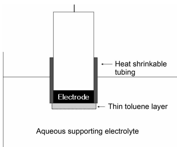
Figure 1. Schematic depiction of the EPG electrode with a thin toluene layer between the electrode surface and aqueous supporting electrolyte.
