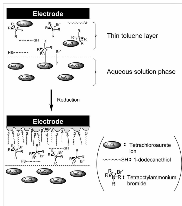
Scheme 1. Schematic descriptions of the transfer of tetrachloroaurate ( \text{AuCl}_4^- ) ions into the thin toluene layer and electro-reduction.
