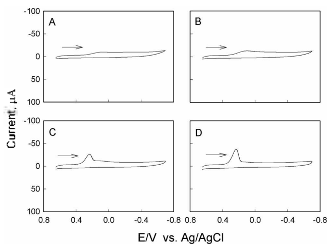
Figure 4. Cyclic voltammograms in 0.1 mM \text{HAuCl}_4 solution at the EPG electrode coated with 10 \mu\text{L} toluene containing 0.05 M TOABr. The voltammograms were obtained at (A) 05, (B) 10, (C) 25, and (D) 35 min after the toluene aliquot was dropped over the electrode surface. The other conditions are the same as those in Figure 2.
