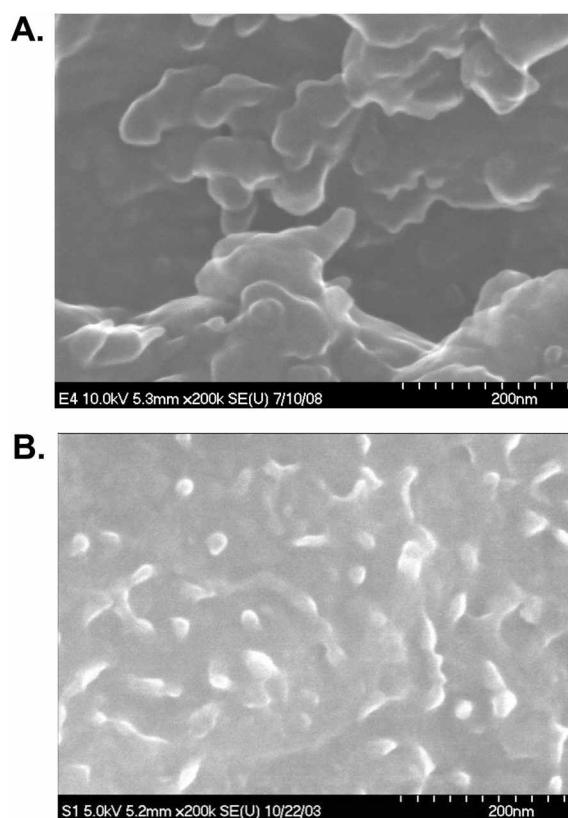
Figure 6. The FE-SEM images of the electro-deposited metallic film on the EPG surface. The samples were prepared by scanning the potential from 0.65 V to -0.7 V in 0.1 mM \text{HAuCl}_4 solution with the EPG electrode, over which an aliquot of 10 \mu\text{L} of toluene containing 0.05 M TOABr was coated. In the toluene layer, the dodecanethiol was absent for (A) and present for (B). After 7 cyclic scans at 5 min intervals, the electrode was taken out of the cell, washed with methanol, and dried to obtain the images.
