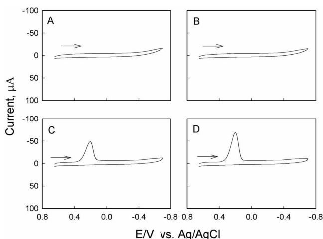
Figure 5. Cyclic voltammograms in 0.1 mM \text{HAuCl}_4 solution at the EPG electrode coated with 10 \mu\text{L} toluene containing 0.05 M TOABr plus 10.4 mM dodecanethiol. The voltammograms were obtained at (A) 05, (B) 10, (C) 25, and (D) 35 min after the toluene aliquot was dropped over the electrode surface. The other conditions are the same as those in Figure 2.
