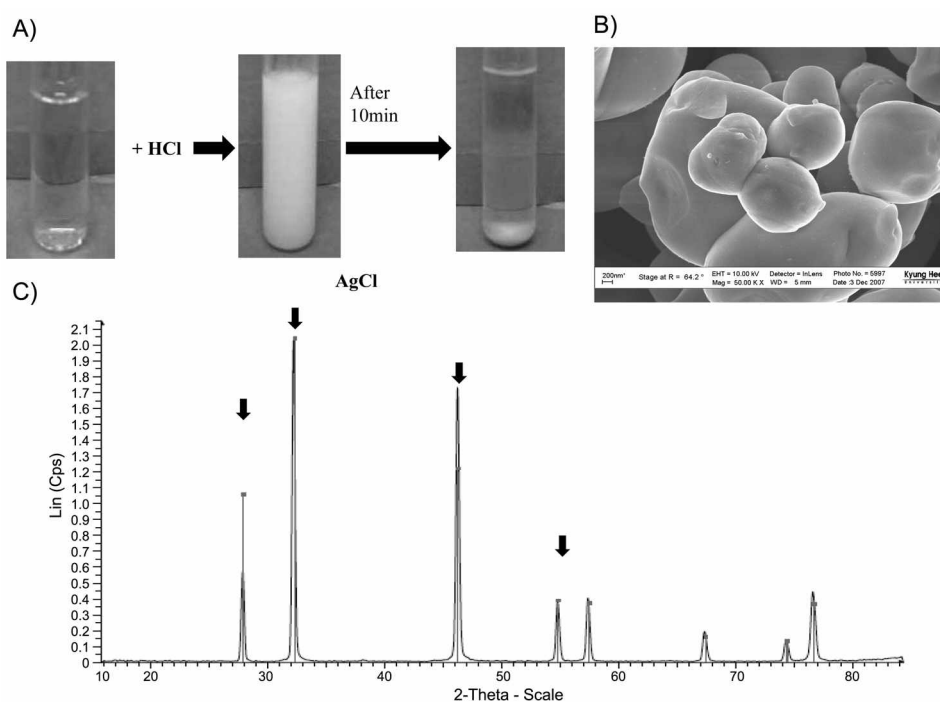
Figure 2. The property of nanometer sized silver materials. The process for the formation of the nano silver precipitate is shown in (A). The FE-SEM analysis of the precipitate (B), the X-RD pattern of the precipitate (C). The sediment analysis yielded \text{AgCl} by X-RD, which suggests the presence of Ag ions in the nanometer the silver solutions.
