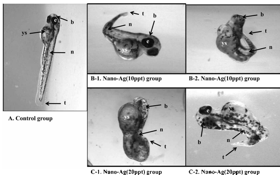
Figure 3. The effects of nanometer sized Ag on the development of zebrafish. Embryos were exposed to Ag 10 ppt (B-1, B-2) and Ag 20 ppt (C-1, C-2). These images show exposed zebrafish at 48 hpf. Abbreviations: b, brain; e, eye; n, notochord; t, tail; ys, yolk sac.
