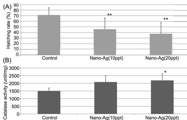
Figure 5. The effects of nanometer sized silver on the hatching rate (A) and catalase activity (B). The hatching rate decreased in groups exposed to nanometer sized silver (10 ppt, 20 ppt) compared to the control group. The catalase activities in the nano-silver exposed groups are also shown to be increased. In particular, the catalase activity in the 20 ppt nano-silver exposed group is significantly greater than that in the control group.
