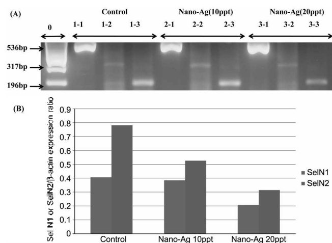
Figure 6. RT-PCR results for the Sel N-1 and Sel N-2 genes in hatched zebrafish under nanometer sized silver exposed conditions (10 ppt and 20 ppt). (A) The line 0 denotes the marker. \beta -actin is at 536 bp, Sel N1 is found at 317 bp and Sel N2 is at 196 bp. The data for the control group are shown in 1-1 ( \beta -actin), 1-2 (Sel N1) and 1-3 (Sel N2). The data for the 10 ppt nanometer sized silver exposed group are 2-1 ( \beta -actin), 2-2 (Sel N1) and 2-3 (Sel N2). The data lines for the 20 ppt nanometer sized silver exposed group are denoted by 3-1 to 3-3. (B) Band intensities of the amplification products were obtained using gel documentation and analysis systems. The gene expression was evaluated relative to \beta -actin. Values are represented as Sel N1 or Sel N2/ \beta -actin expression ratios in zebrafish ( n = 30 ).
