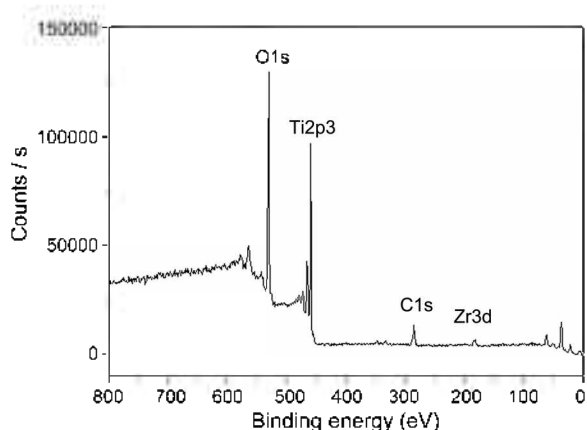
Figure 9. XPS spectrum of 3 wt % Zr-TiO 2 -S calcined at 450 °C.
