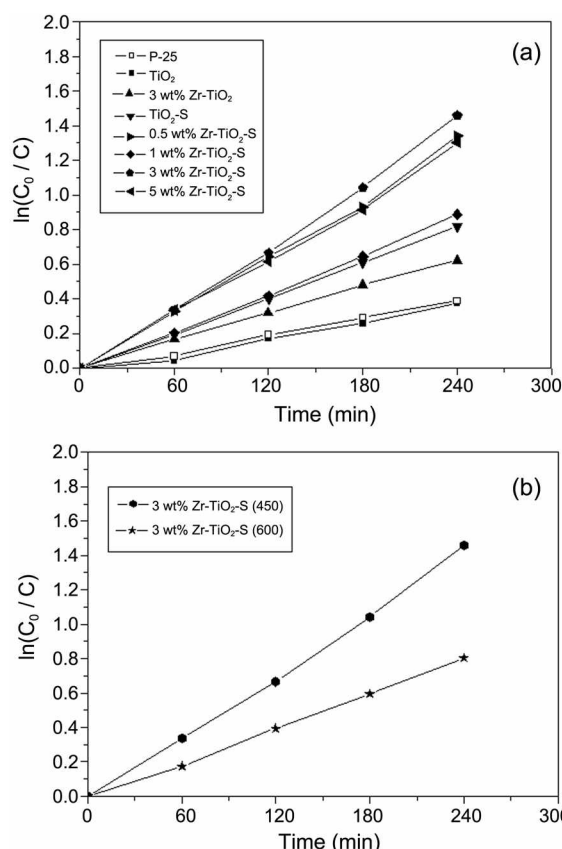
Figure 11. Photocatalytic degradation of toluene under visible light irradiation: (a) various catalysts calcined at 450 °C and (b) 3 wt % Zr-TiO 2 -S calcined at 450 °C or 600 °C. C 0 = the initial concentration, C = the concentration at time t.
