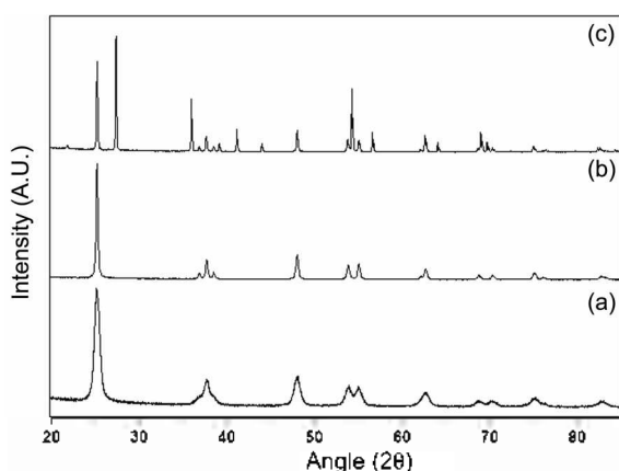
Figure 4. XRD patterns of 3 wt % Zr-TiO 2 -S calcined at (a) 600 °C, (b) 800 °C and (c) 900 °C.
