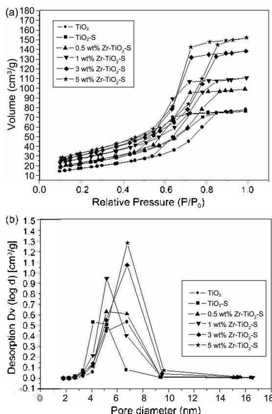
Figure 6. Textural properties of catalysts calcined at 450 °C: (a) N 2 adsorption-desorption isotherms and (b) BJH pore-size distribution curves.
